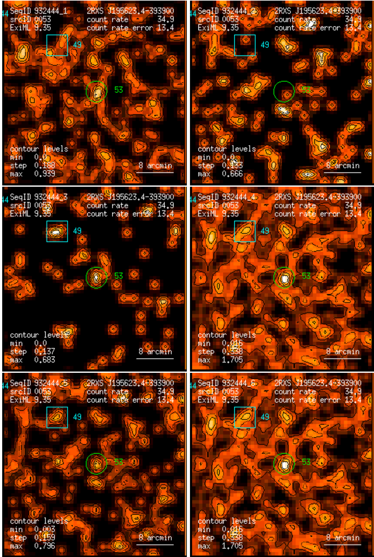
Figure 53: RASS 932444: detection 0053: band rate images, Gaussian filter: (1) PSPC channels 11 – 41, (2) 52 – 90, (3) 91 – 201, (4) 11 – 235, (5) 52 – 201, (6) 11 – 201. Broad band rates in counts/ks. Band rate contour levels in counts/ks/arcmin 2 .
