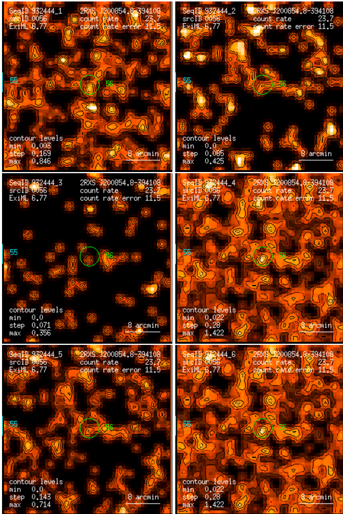
Figure 56: RASS 932444: detection 0056: band rate images, Gaussian filter: (1) PSPC channels 11 – 41, (2) 52 – 90, (3) 91 – 201, (4) 11 – 235, (5) 52 – 201, (6) 11 – 201. Broad band rates in counts/ks. Band rate contour levels in counts/ks/arcmin 2 .
