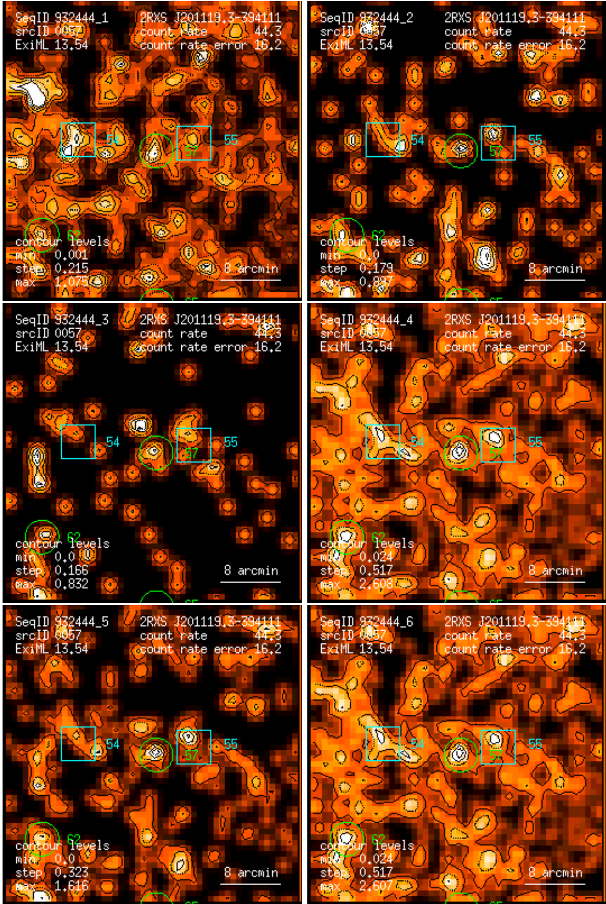
Figure 57: RASS 932444: detection 0057: band rate images, Gaussian filter: (1) PSPC channels 11 – 41, (2) 52 – 90, (3) 91 – 201, (4) 11 – 235, (5) 52 – 201, (6) 11 – 201. Broad band rates in counts/ks. Band rate contour levels in counts/ks/arcmin 2 .
