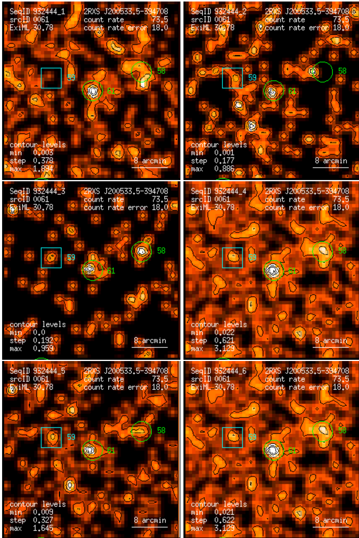
Figure 61: RASS 932444: detection 0061: band rate images, Gaussian filter: (1) PSPC channels 11 – 41, (2) 52 – 90, (3) 91 – 201, (4) 11 – 235, (5) 52 – 201, (6) 11 – 201. Broad band rates in counts/ks. Band rate contour levels in counts/ks/arcmin 2 .
