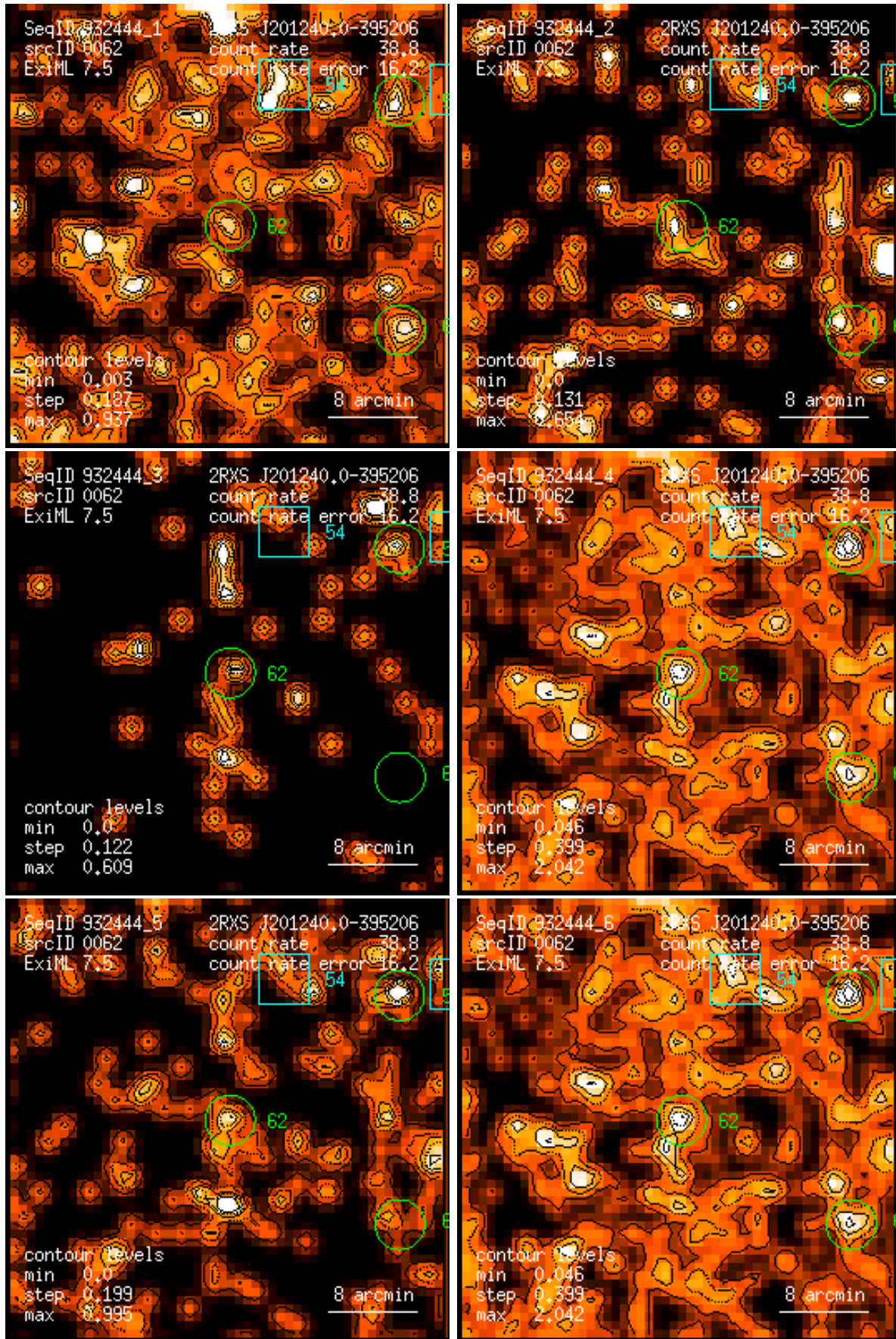
Figure 62: RASS 932444: detection 0062: band rate images, Gaussian filter: (1) PSPC channels 11 – 41, (2) 52 – 90, (3) 91 – 201, (4) 11 – 235, (5) 52 – 201, (6) 11 – 201. Broad band rates in counts/ks. Band rate contour levels in counts/ks/arcmin 2 .
