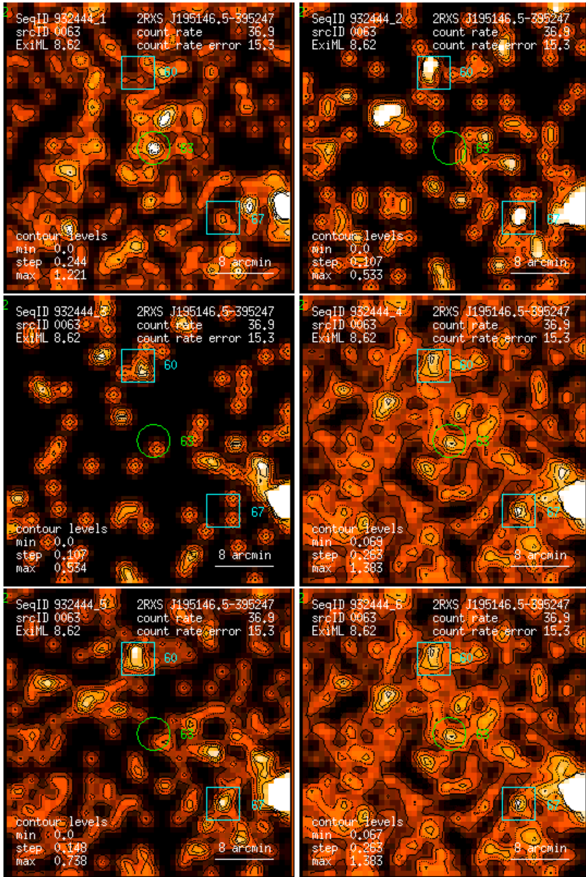
Figure 63: RASS 932444: detection 0063: band rate images, Gaussian filter: (1) PSPC channels 11 – 41, (2) 52 – 90, (3) 91 – 201, (4) 11 – 235, (5) 52 – 201, (6) 11 – 201. Broad band rates in counts/ks. Band rate contour levels in counts/ks/arcmin 2 .
