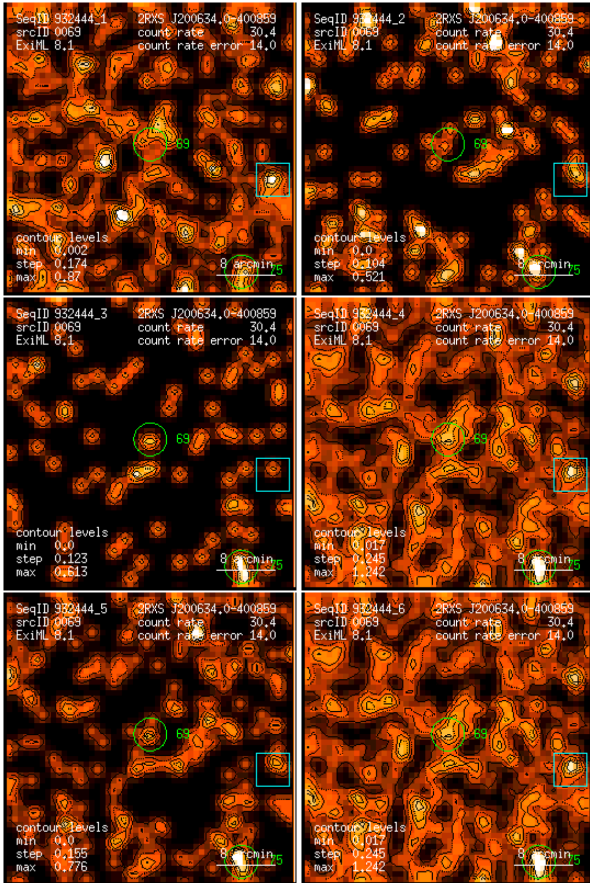
Figure 69: RASS 932444: detection 0069: band rate images, Gaussian filter: (1) PSPC channels 11 – 41, (2) 52 – 90, (3) 91 – 201, (4) 11 – 235, (5) 52 – 201, (6) 11 – 201. Broad band rates in counts/ks. Band rate contour levels in counts/ks/arcmin 2 .
