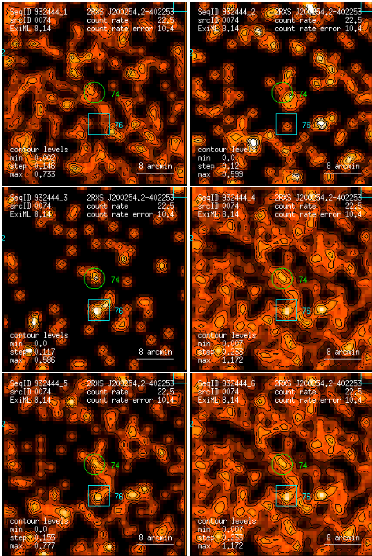
Figure 74: RASS 932444: detection 0074: band rate images, Gaussian filter: (1) PSPC channels 11 – 41, (2) 52 – 90, (3) 91 – 201, (4) 11 – 235, (5) 52 – 201, (6) 11 – 201. Broad band rates in counts/ks. Band rate contour levels in counts/ks/arcmin 2 .
