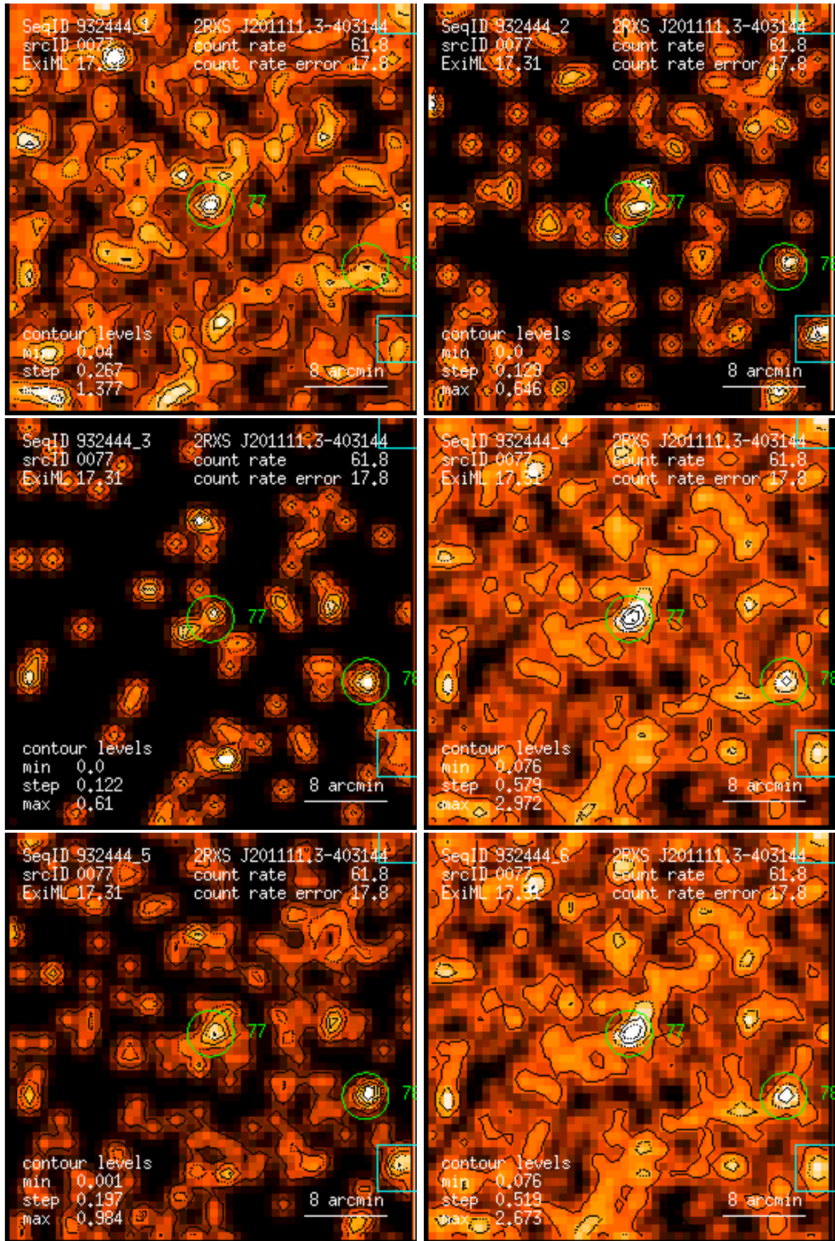
Figure 77: RASS 932444: detection 0077: band rate images, Gaussian filter: (1) PSPC channels 11 – 41, (2) 52 – 90, (3) 91 – 201, (4) 11 – 235, (5) 52 – 201, (6) 11 – 201. Broad band rates in counts/ks. Band rate contour levels in counts/ks/arcmin 2 .
