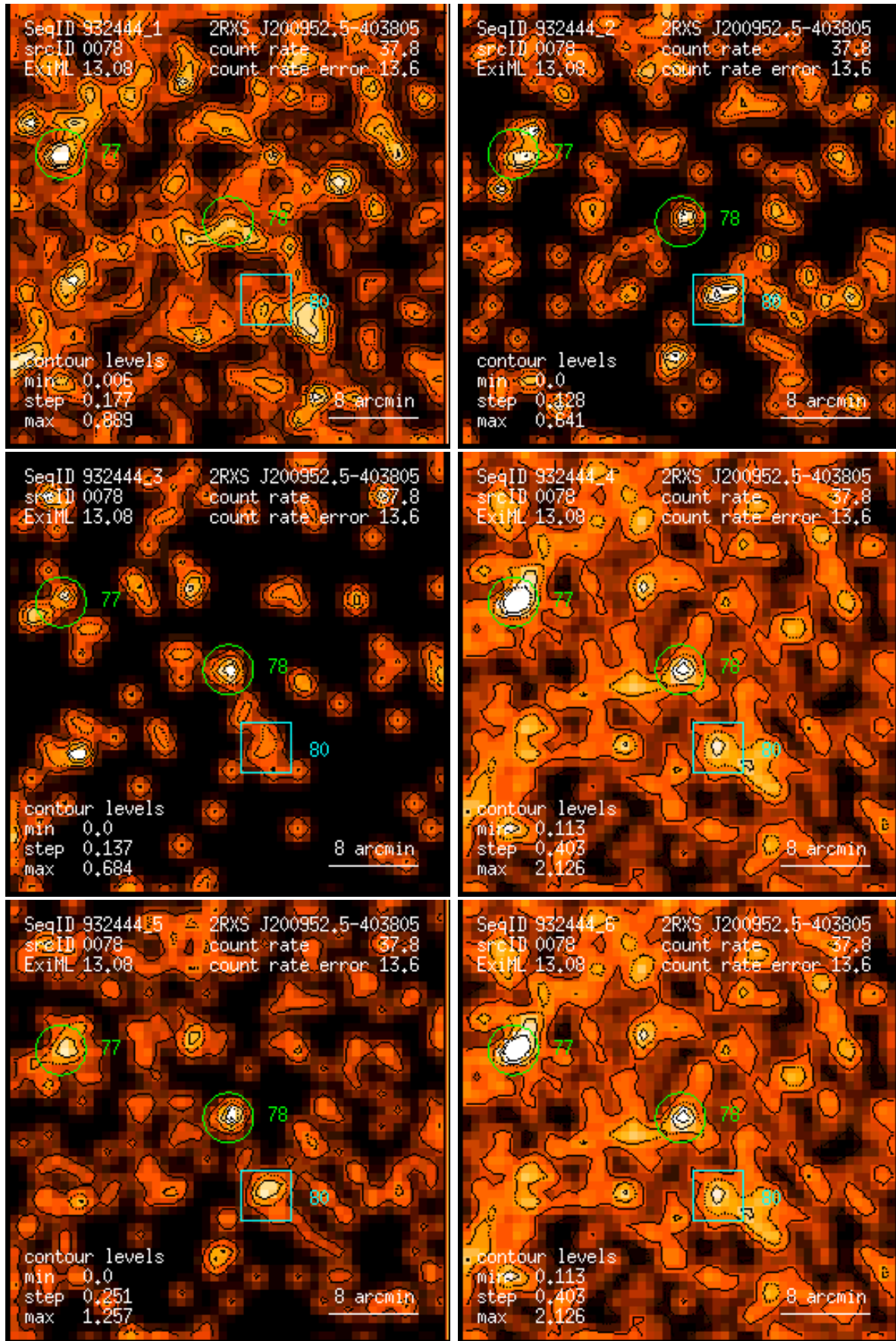
Figure 78: RASS 932444: detection 0078: band rate images, Gaussian filter: (1) PSPC channels 11 – 41, (2) 52 – 90, (3) 91 – 201, (4) 11 – 235, (5) 52 – 201, (6) 11 – 201. Broad band rates in counts/ks. Band rate contour levels in counts/ks/arcmin 2 .
