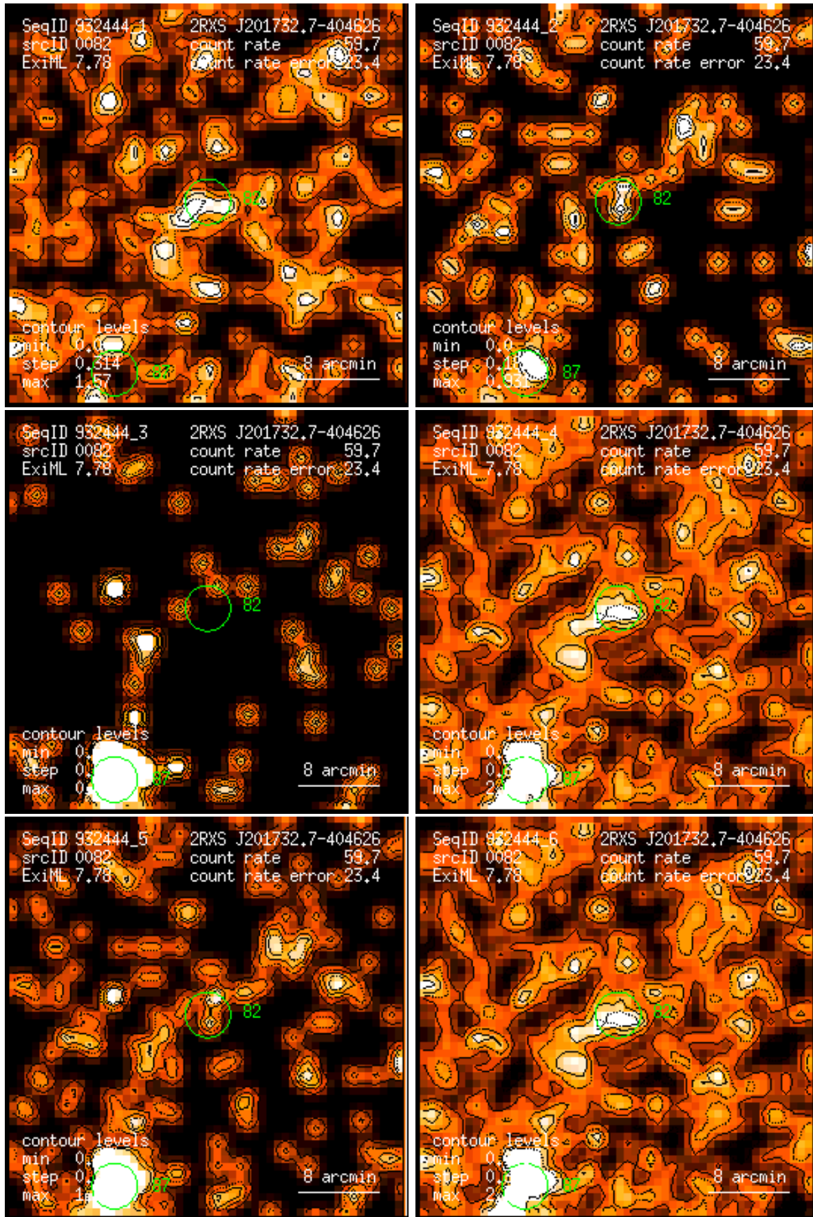
Figure 82: RASS 932444: detection 0082: band rate images, Gaussian filter: (1) PSPC channels 11 – 41, (2) 52 – 90, (3) 91 – 201, (4) 11 – 235, (5) 52 – 201, (6) 11 – 201. Broad band rates in counts/ks. Band rate contour levels in counts/ks/arcmin 2 .
