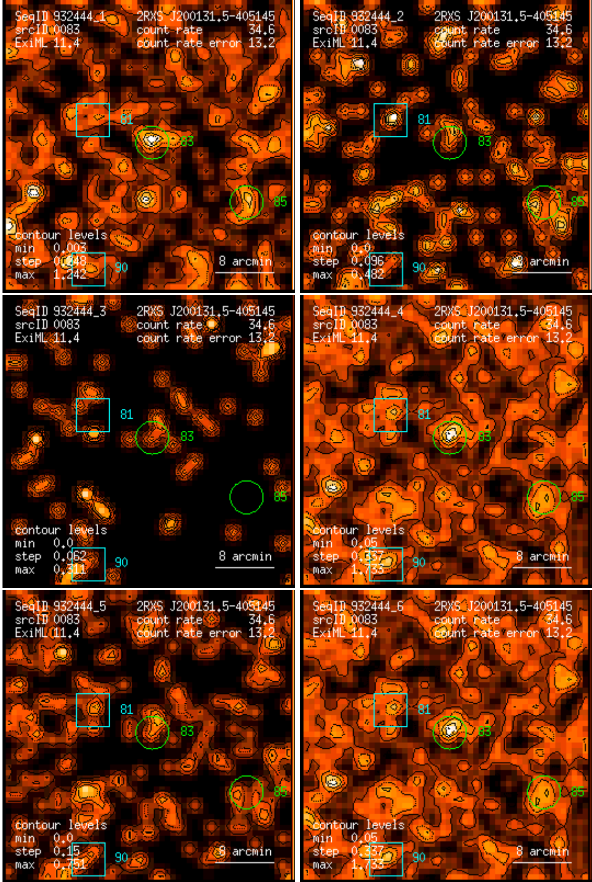
Figure 83: RASS 932444: detection 0083: band rate images, Gaussian filter: (1) PSPC channels 11 – 41, (2) 52 – 90, (3) 91 – 201, (4) 11 – 235, (5) 52 – 201, (6) 11 – 201. Broad band rates in counts/ks. Band rate contour levels in counts/ks/arcmin 2 .
