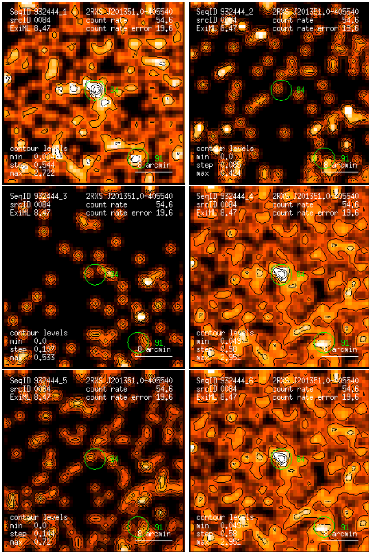
Figure 84: RASS 932444: detection 0084: band rate images, Gaussian filter: (1) PSPC channels 11 – 41, (2) 52 – 90, (3) 91 – 201, (4) 11 – 235, (5) 52 – 201, (6) 11 – 201. Broad band rates in counts/ks. Band rate contour levels in counts/ks/arcmin 2 .
