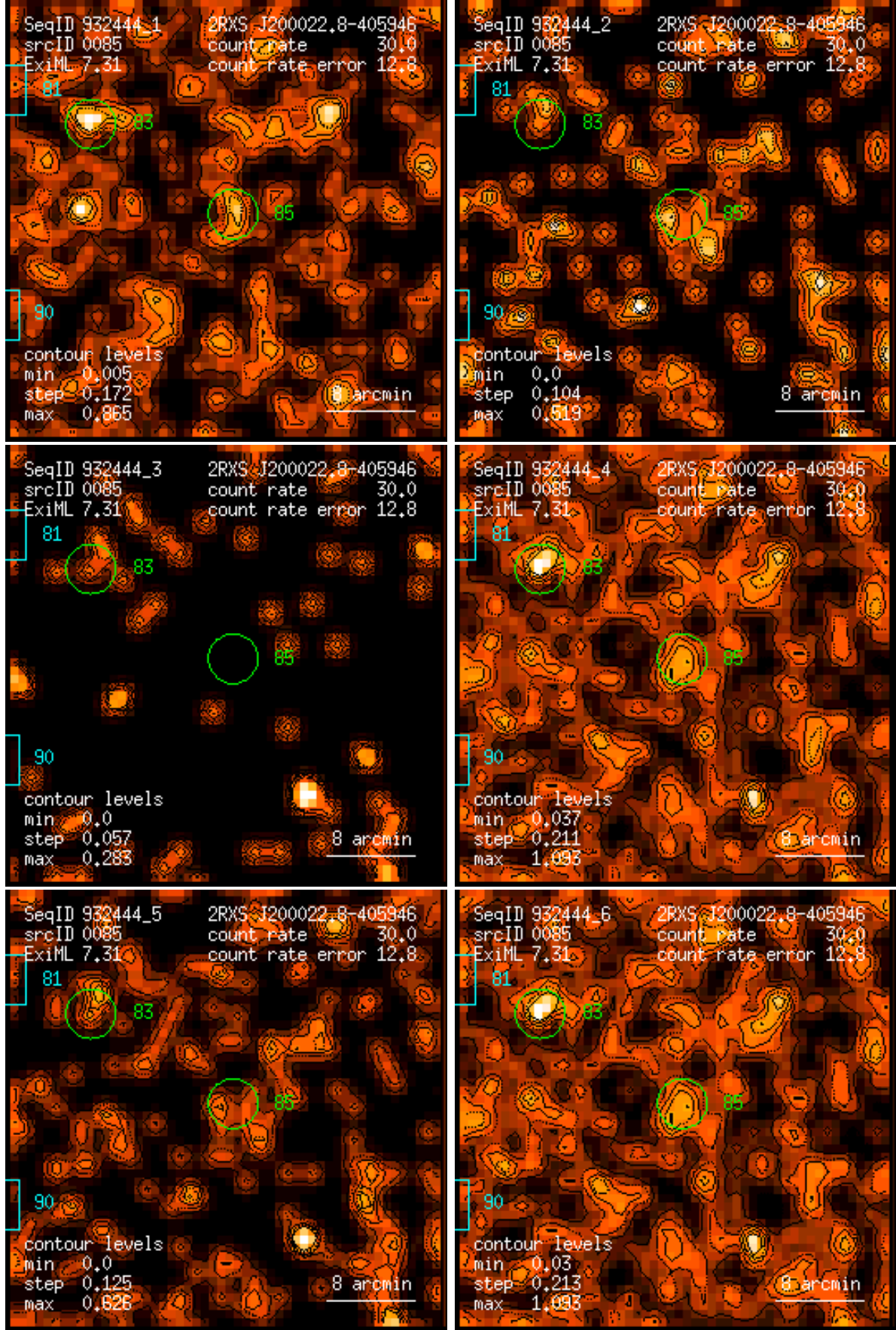
Figure 85: RASS 932444: detection 0085: band rate images, Gaussian filter: (1) PSPC channels 11 – 41, (2) 52 – 90, (3) 91 – 201, (4) 11 – 235, (5) 52 – 201, (6) 11 – 201. Broad band rates in counts/ks. Band rate contour levels in counts/ks/arcmin 2 .
