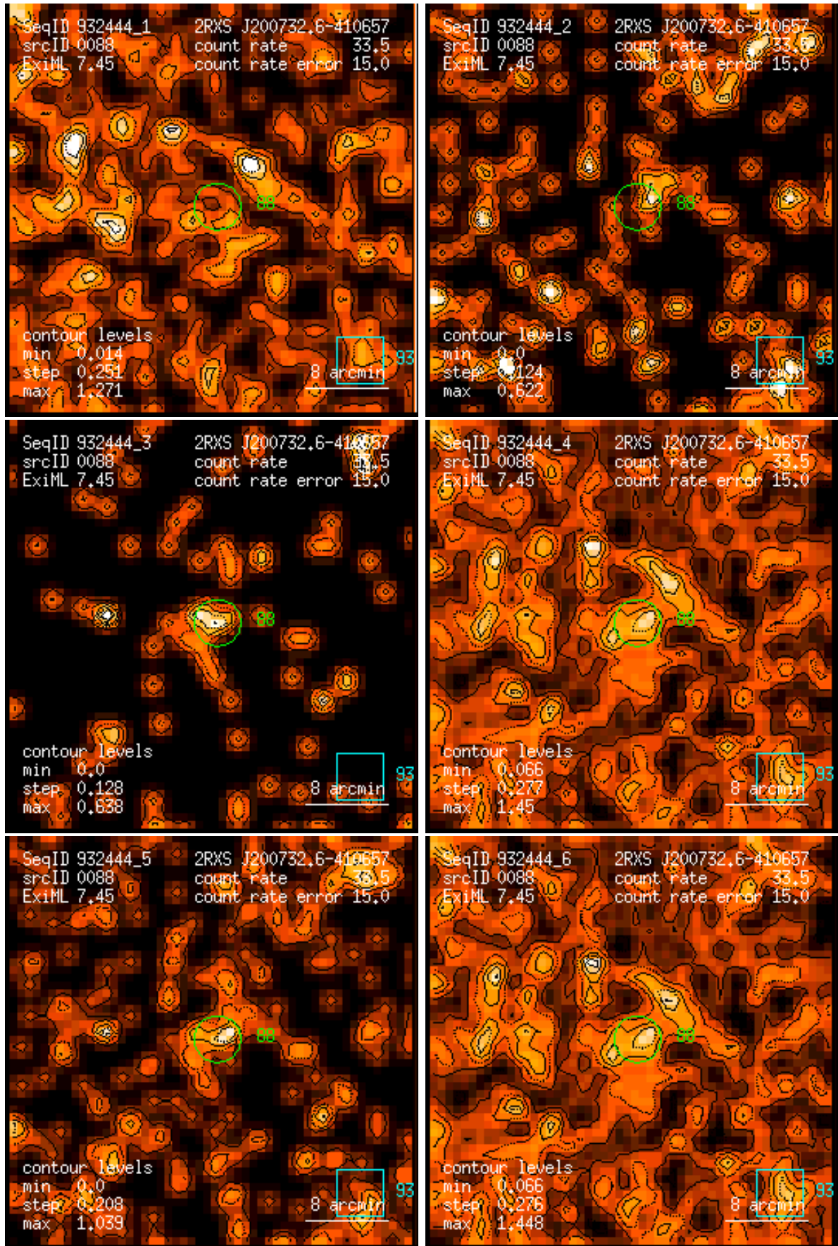
Figure 88: RASS 932444: detection 0088: band rate images, Gaussian filter: (1) PSPC channels 11 – 41, (2) 52 – 90, (3) 91 – 201, (4) 11 – 235, (5) 52 – 201, (6) 11 – 201. Broad band rates in counts/ks. Band rate contour levels in counts/ks/arcmin 2 .
