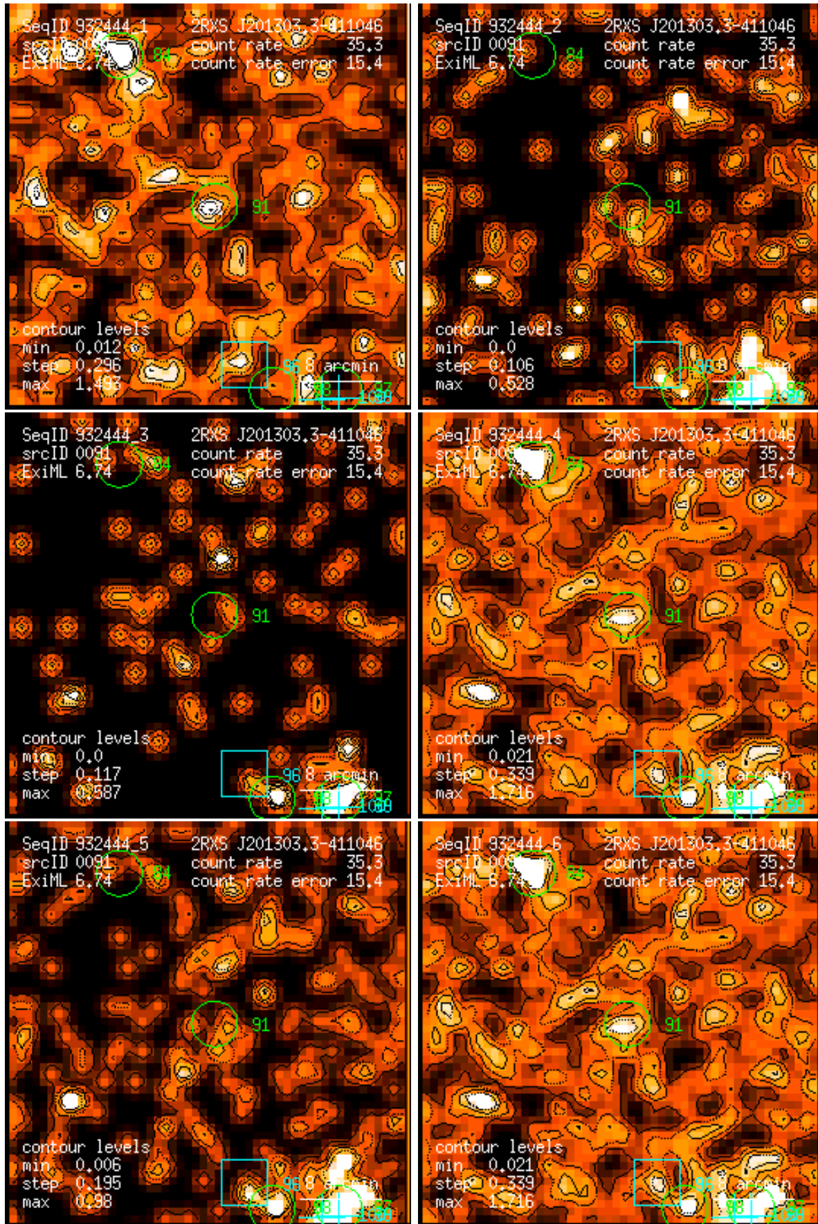
Figure 91: RASS 932444: detection 0091: band rate images, Gaussian filter: (1) PSPC channels 11 – 41, (2) 52 – 90, (3) 91 – 201, (4) 11 – 235, (5) 52 – 201, (6) 11 – 201. Broad band rates in counts/ks. Band rate contour levels in counts/ks/arcmin 2 .
