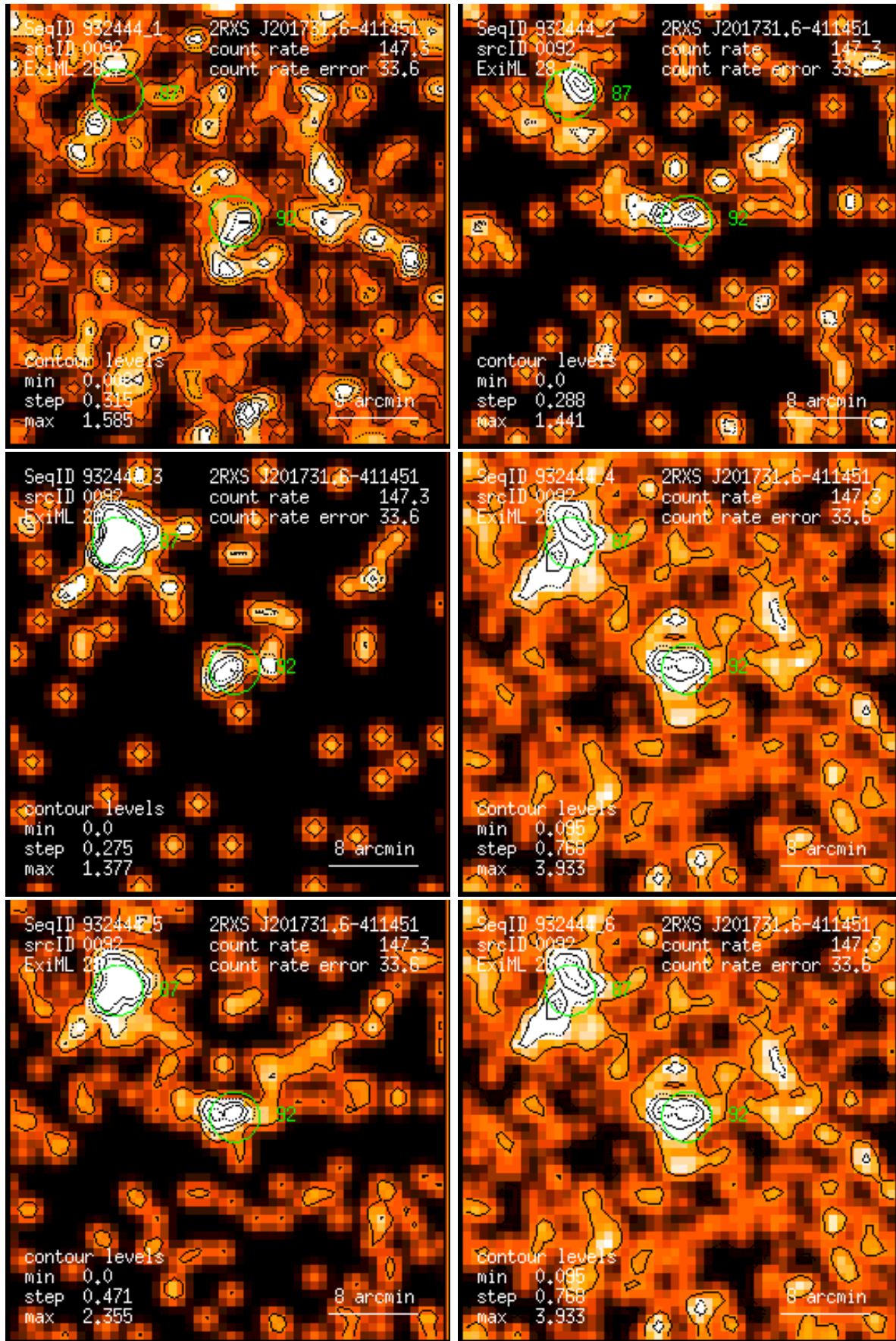
Figure 92: RASS 932444: detection 0092: band rate images, Gaussian filter: (1) PSPC channels 11 – 41, (2) 52 – 90, (3) 91 – 201, (4) 11 – 235, (5) 52 – 201, (6) 11 – 201. Broad band rates in counts/ks. Band rate contour levels in counts/ks/arcmin 2 .
