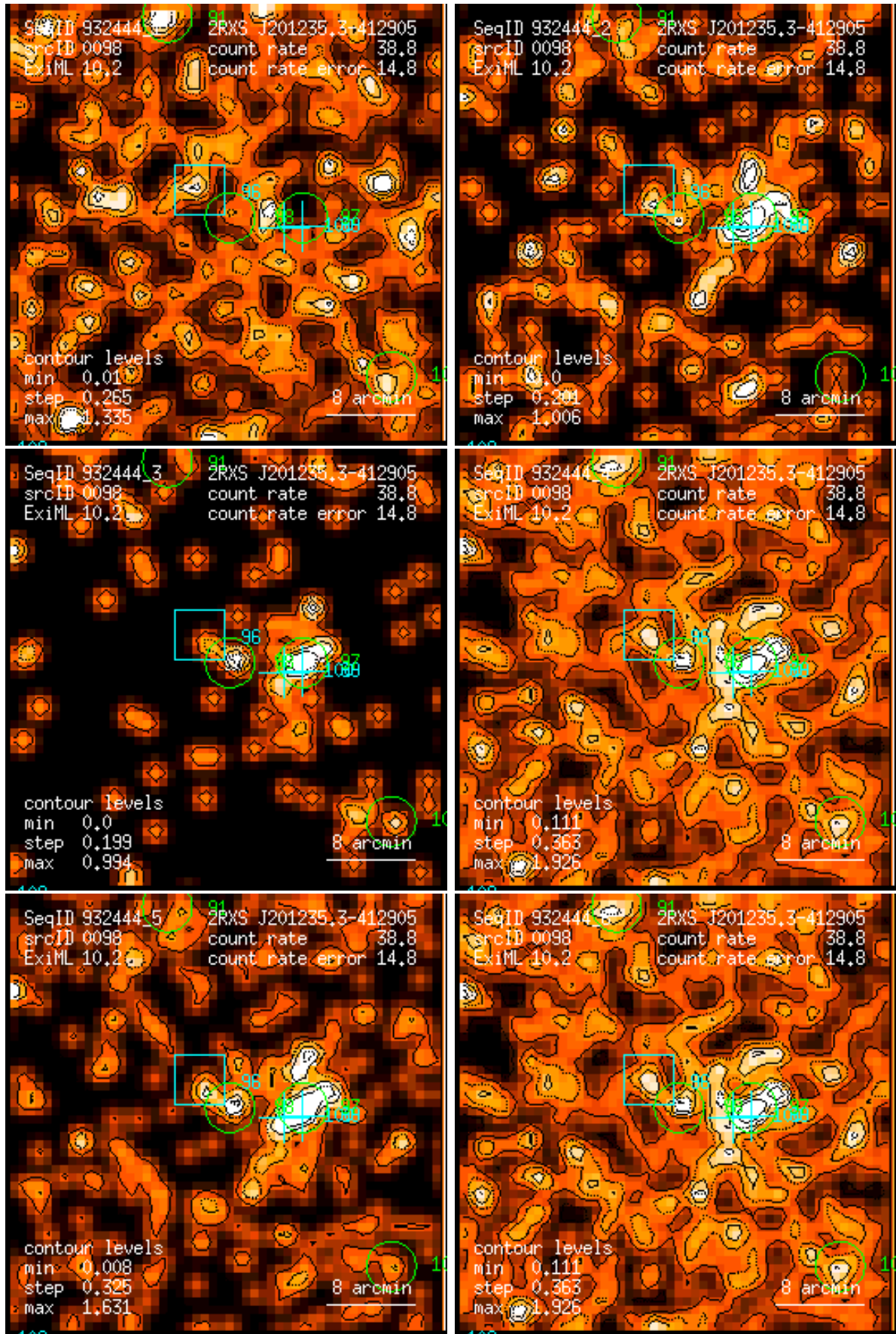
Figure 98: RASS 932444: detection 0098: band rate images, Gaussian filter: (1) PSPC channels 11 – 41, (2) 52 – 90, (3) 91 – 201, (4) 11 – 235, (5) 52 – 201, (6) 11 – 201. Broad band rates in counts/ks. Band rate contour levels in counts/ks/arcmin 2 .
