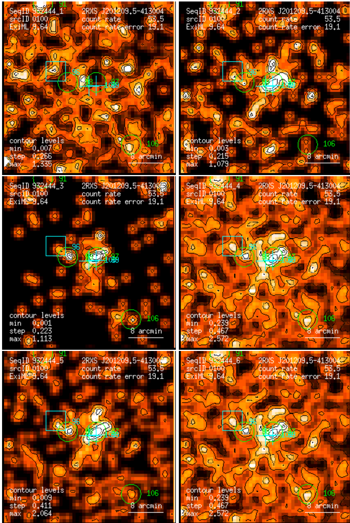
Figure 100: RASS 932444: detection 0100: band rate images, Gaussian filter: (1) PSPC channels 11 – 41, (2) 52 – 90, (3) 91 – 201, (4) 11 – 235, (5) 52 – 201, (6) 11 – 201. Broad band rates in counts/ks. Band rate contour levels in counts/ks/arcmin 2 .
