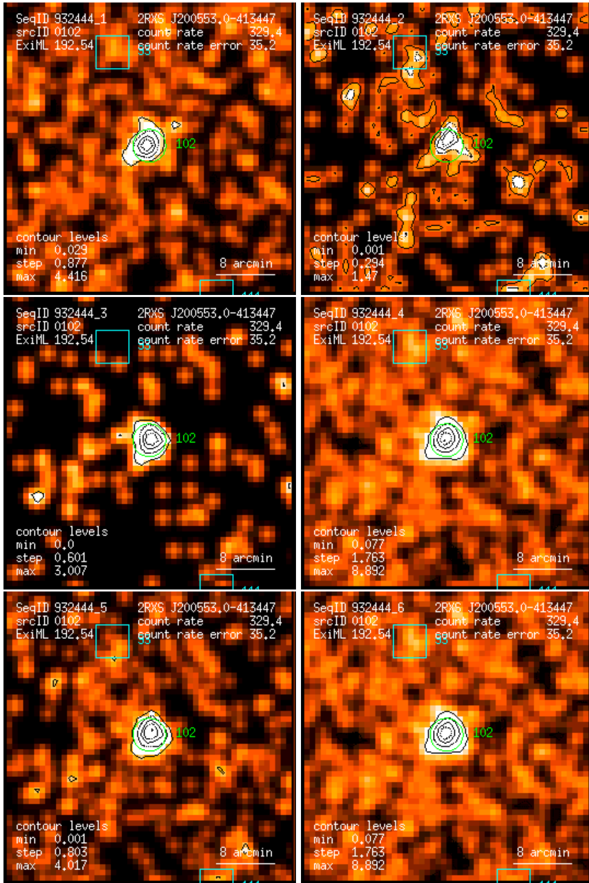
Figure 102: RASS 932444: detection 0102: band rate images, Gaussian filter: (1) PSPC channels 11 – 41, (2) 52 – 90, (3) 91 – 201, (4) 11 – 235, (5) 52 – 201, (6) 11 – 201. Broad band rates in counts/ks. Band rate contour levels in counts/ks/arcmin 2 .
