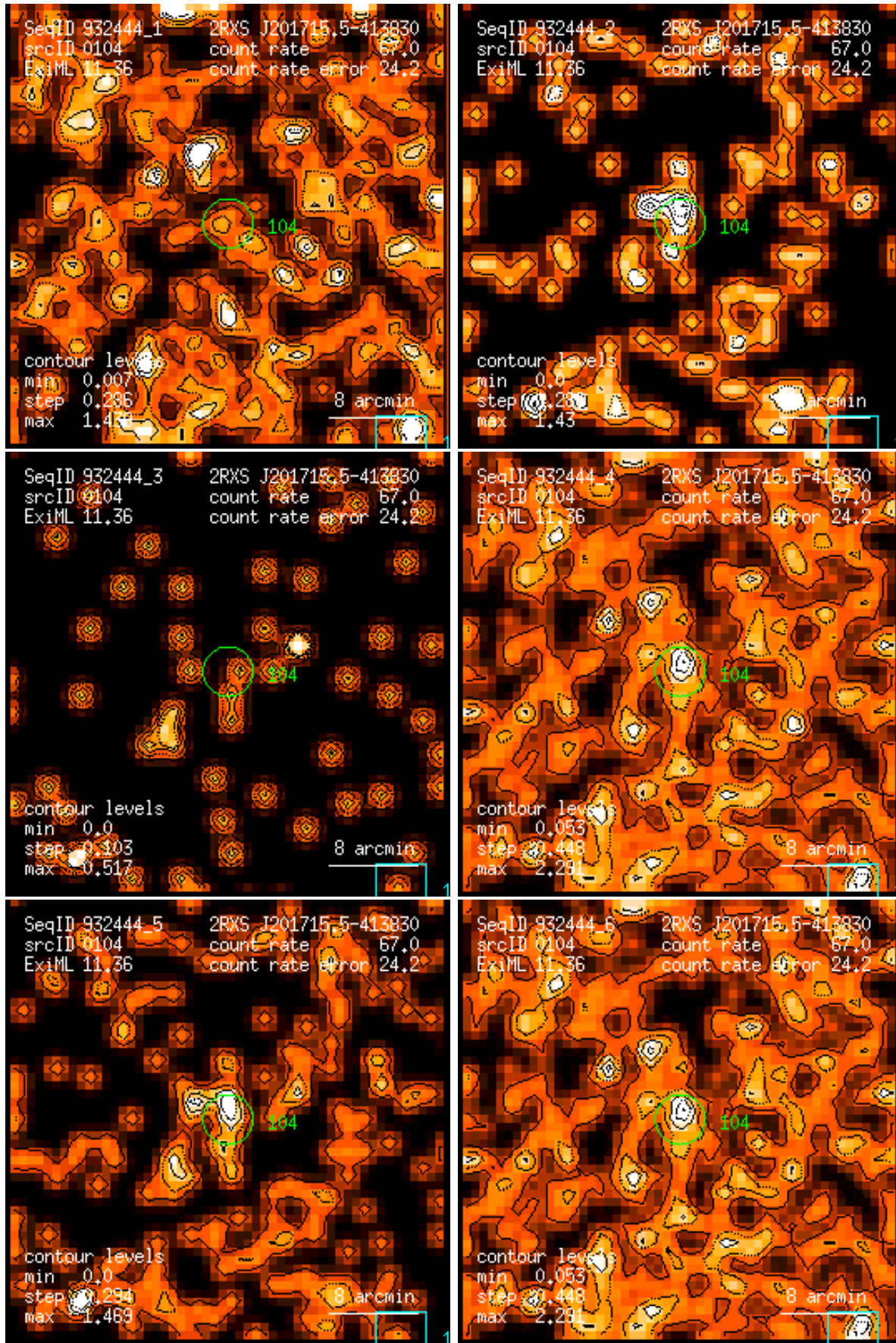
Figure 104: RASS 932444: detection 0104: band rate images, Gaussian filter: (1) PSPC channels 11 – 41, (2) 52 – 90, (3) 91 – 201, (4) 11 – 235, (5) 52 – 201, (6) 11 – 201. Broad band rates in counts/ks. Band rate contour levels in counts/ks/arcmin 2 .
