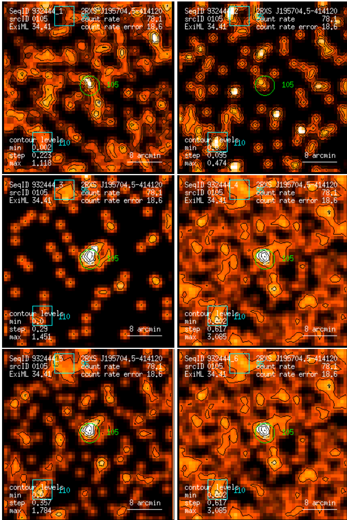
Figure 105: RASS 932444: detection 0105: band rate images, Gaussian filter: (1) PSPC channels 11 – 41, (2) 52 – 90, (3) 91 – 201, (4) 11 – 235, (5) 52 – 201, (6) 11 – 201. Broad band rates in counts/ks. Band rate contour levels in counts/ks/arcmin 2 .
