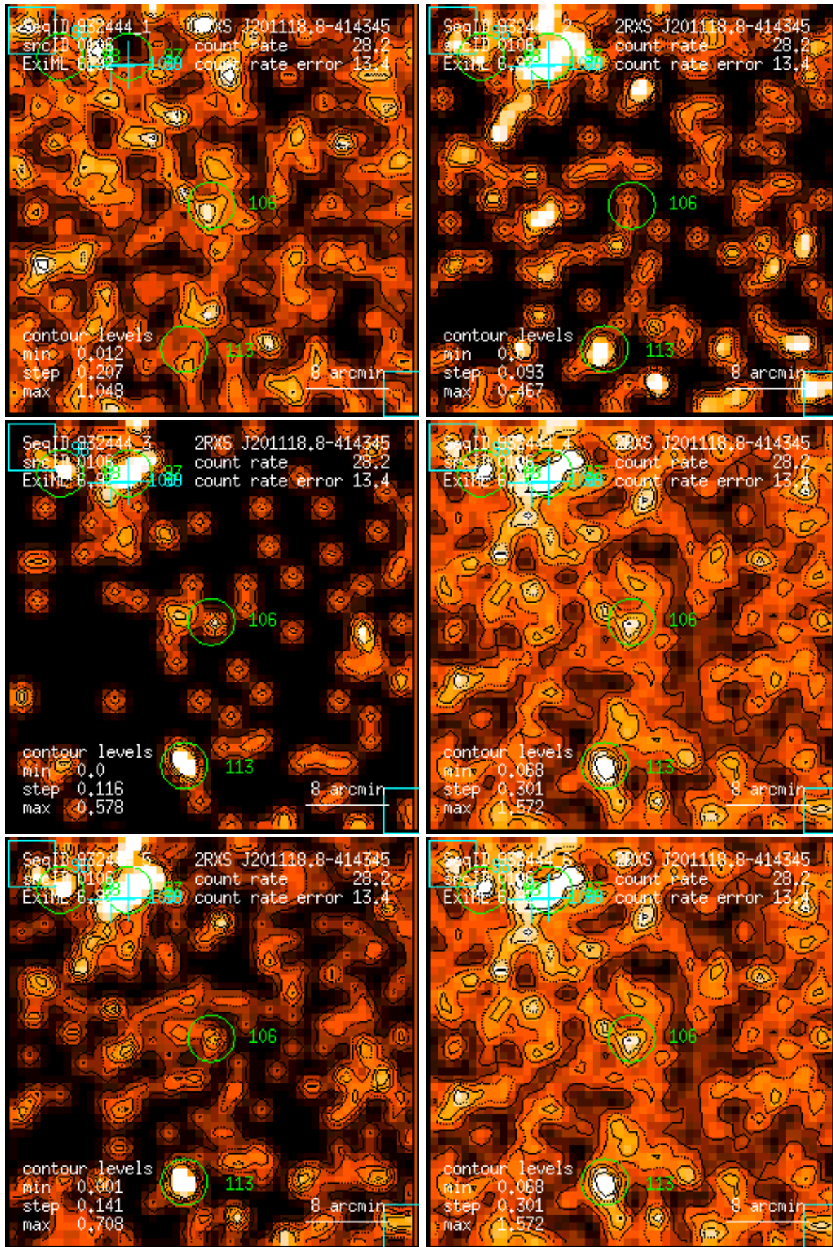
Figure 106: RASS 932444: detection 0106: band rate images, Gaussian filter: (1) PSPC channels 11 – 41, (2) 52 – 90, (3) 91 – 201, (4) 11 – 235, (5) 52 – 201, (6) 11 – 201. Broad band rates in counts/ks. Band rate contour levels in counts/ks/arcmin 2 .
