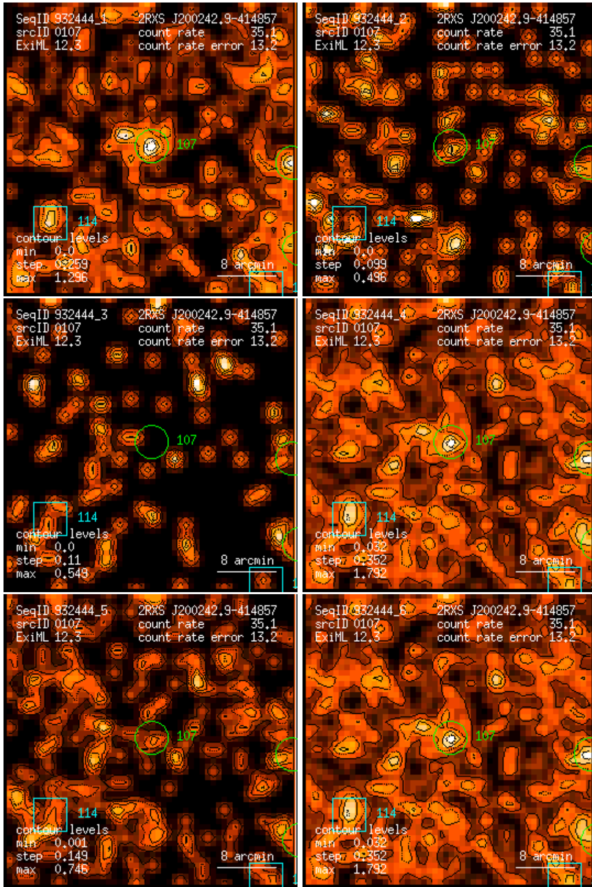
Figure 107: RASS 932444: detection 0107: band rate images, Gaussian filter: (1) PSPC channels 11 – 41, (2) 52 – 90, (3) 91 – 201, (4) 11 – 235, (5) 52 – 201, (6) 11 – 201. Broad band rates in counts/ks. Band rate contour levels in counts/ks/arcmin 2 .
