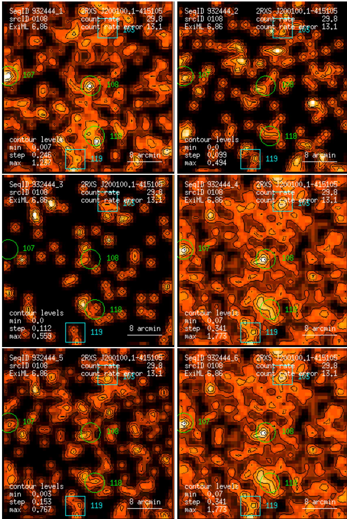
Figure 108: RASS 932444: detection 0108: band rate images, Gaussian filter: (1) PSPC channels 11 – 41, (2) 52 – 90, (3) 91 – 201, (4) 11 – 235, (5) 52 – 201, (6) 11 – 201. Broad band rates in counts/ks. Band rate contour levels in counts/ks/arcmin 2 .
