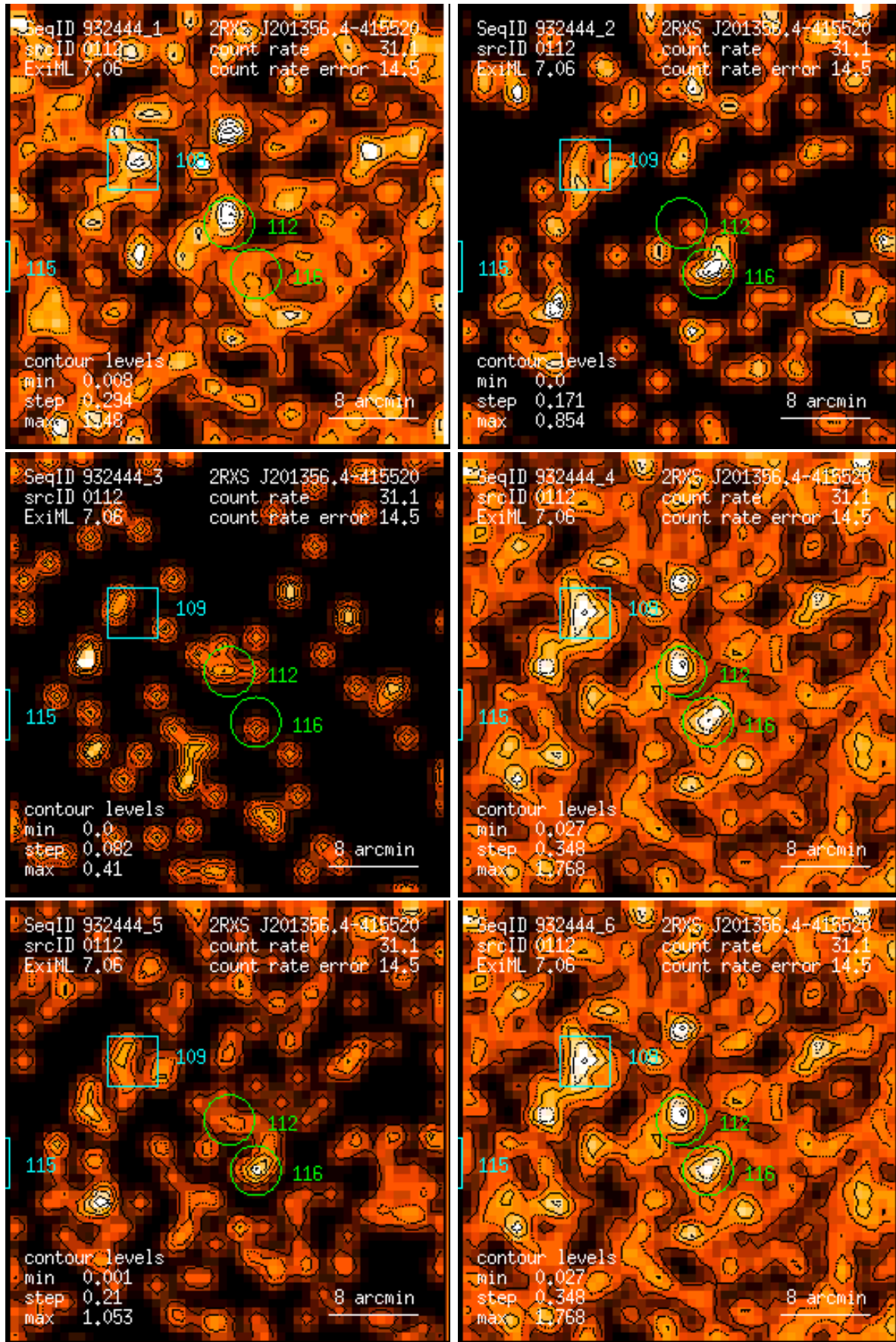
Figure 112: RASS 932444: detection 0112: band rate images, Gaussian filter: (1) PSPC channels 11 – 41, (2) 52 – 90, (3) 91 – 201, (4) 11 – 235, (5) 52 – 201, (6) 11 – 201. Broad band rates in counts/ks. Band rate contour levels in counts/ks/arcmin 2 .
