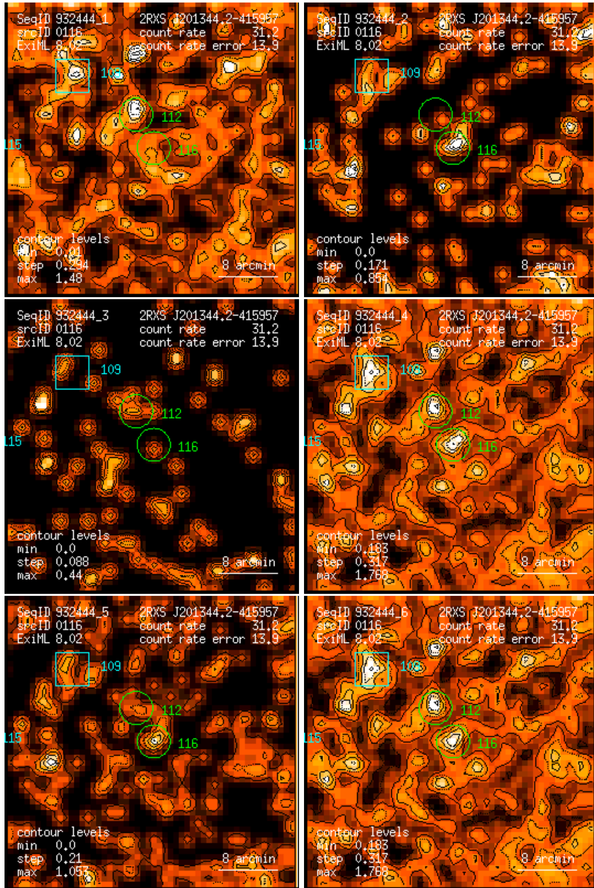
Figure 116: RASS 932444: detection 0116: band rate images, Gaussian filter: (1) PSPC channels 11 – 41, (2) 52 – 90, (3) 91 – 201, (4) 11 – 235, (5) 52 – 201, (6) 11 – 201. Broad band rates in counts/ks. Band rate contour levels in counts/ks/arcmin 2 .
