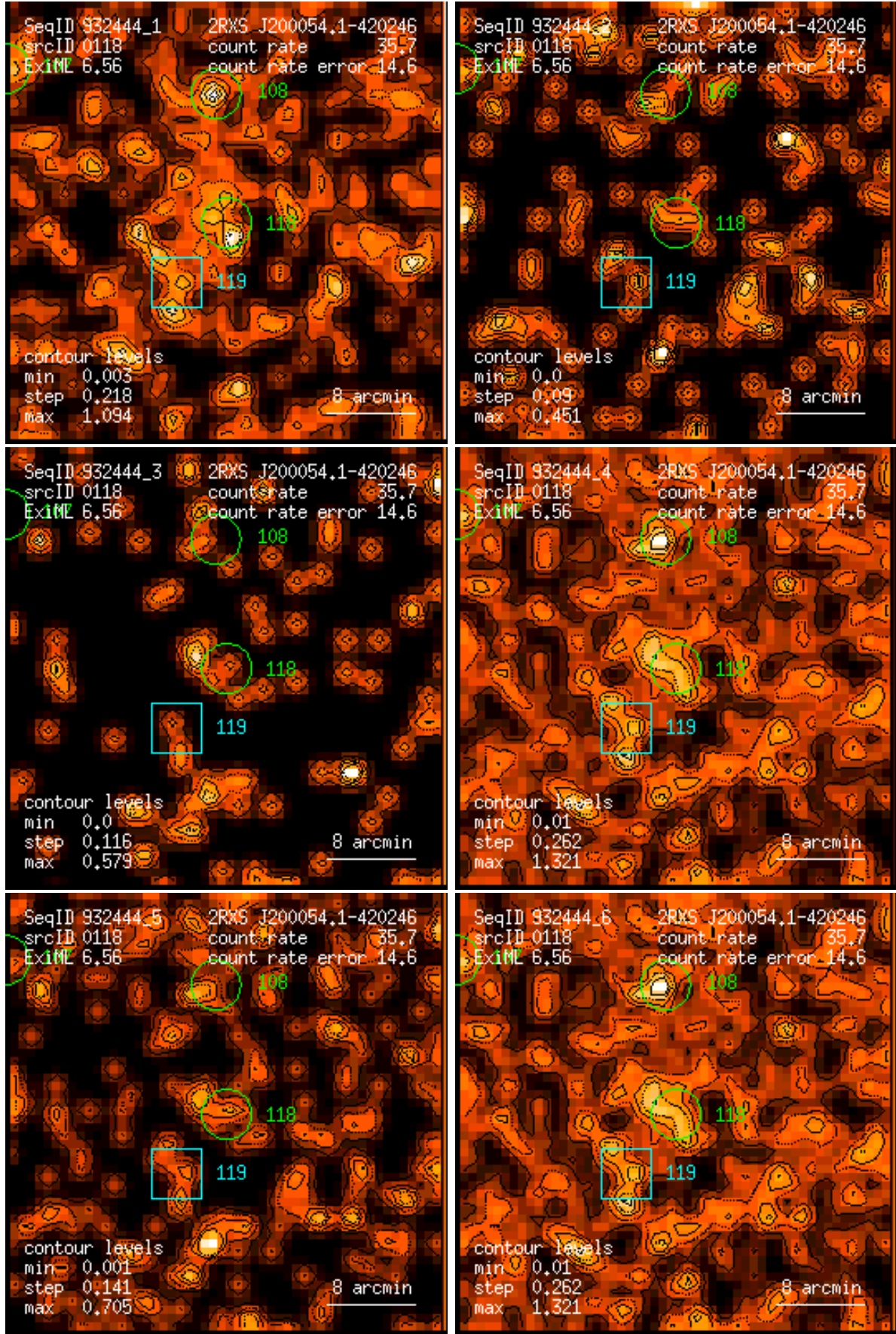
Figure 118: RASS 932444: detection 0118: band rate images, Gaussian filter: (1) PSPC channels 11 – 41, (2) 52 – 90, (3) 91 – 201, (4) 11 – 235, (5) 52 – 201, (6) 11 – 201. Broad band rates in counts/ks. Band rate contour levels in counts/ks/arcmin 2 .
