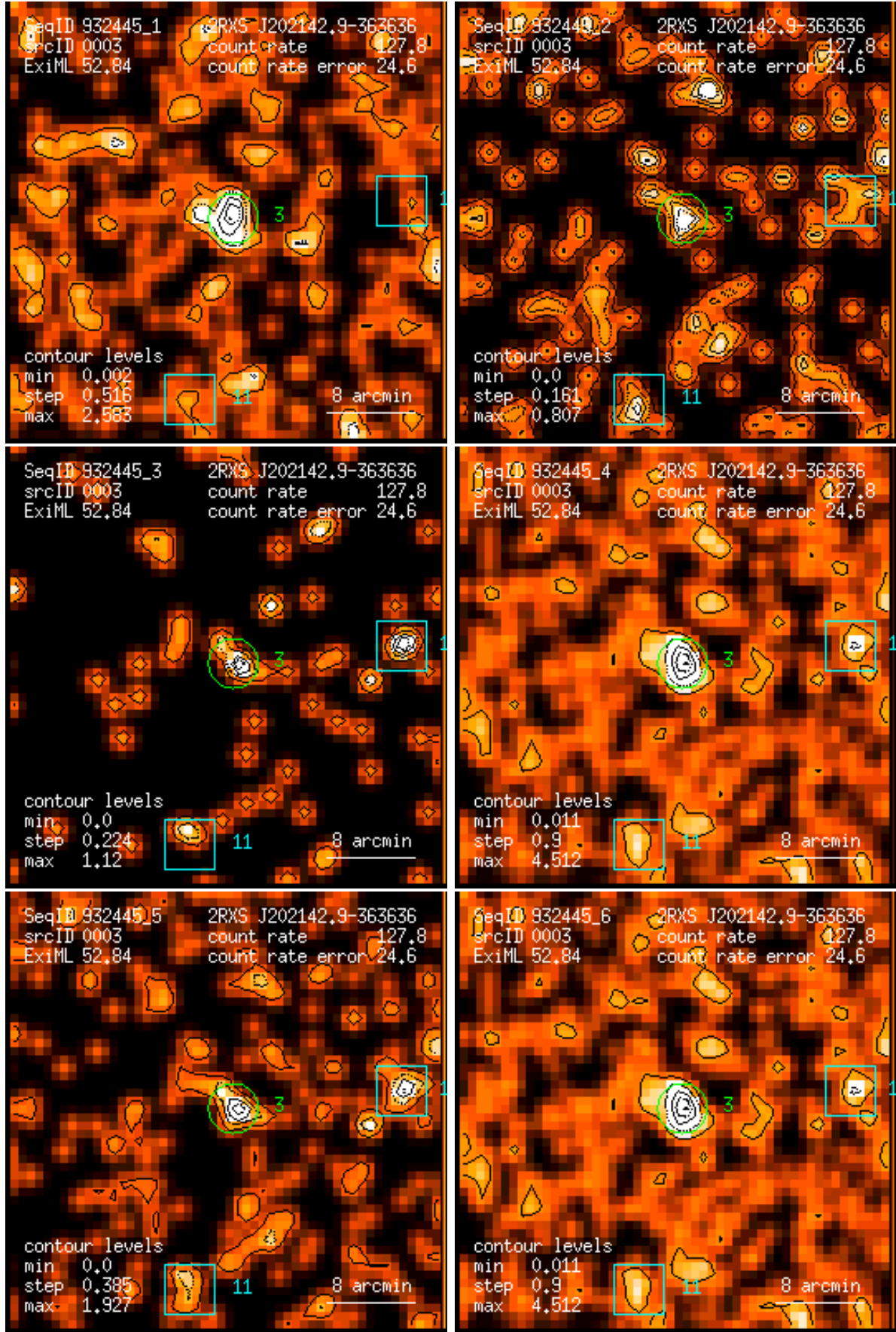
Figure 3: RASS 932445: detection 0003: band rate images, Gaussian filter: (1) PSPC channels 11 – 41, (2) 52 – 90, (3) 91 – 201, (4) 11 – 235, (5) 52 – 201, (6) 11 – 201. Broad band rates in counts/ks. Band rate contour levels in counts/ks/arcmin 2 .
