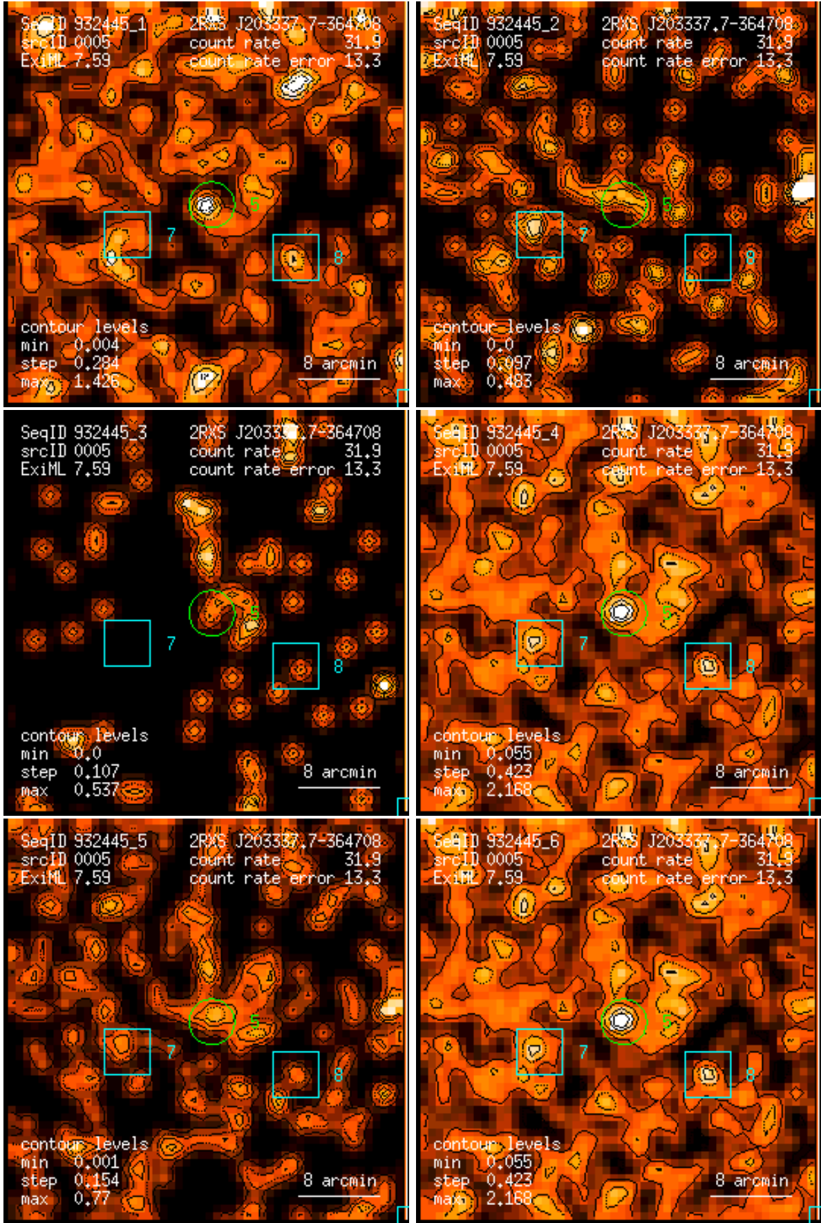
Figure 5: RASS 932445: detection 0005: band rate images, Gaussian filter: (1) PSPC channels 11 – 41, (2) 52 – 90, (3) 91 – 201, (4) 11 – 235, (5) 52 – 201, (6) 11 – 201. Broad band rates in counts/ks. Band rate contour levels in counts/ks/arcmin 2 .
