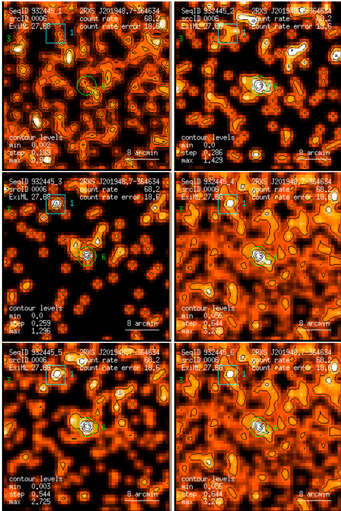
Figure 6: RASS 932445: detection 0006: band rate images, Gaussian filter: (1) PSPC channels 11 – 41, (2) 52 – 90, (3) 91 – 201, (4) 11 – 235, (5) 52 – 201, (6) 11 – 201. Broad band rates in counts/ks. Band rate contour levels in counts/ks/arcmin 2 .
