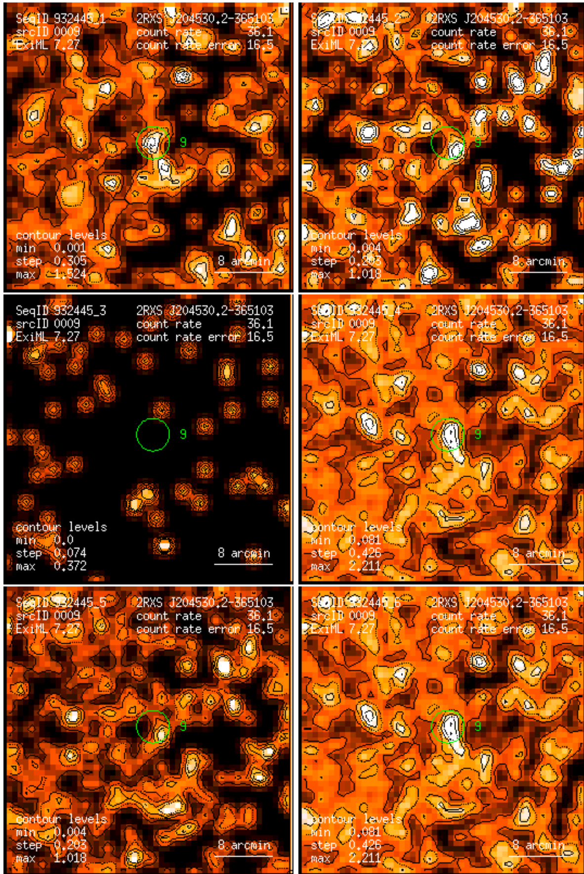
Figure 9: RASS 932445: detection 0009: band rate images, Gaussian filter: (1) PSPC channels 11 – 41, (2) 52 – 90, (3) 91 – 201, (4) 11 – 235, (5) 52 – 201, (6) 11 – 201. Broad band rates in counts/ks. Band rate contour levels in counts/ks/arcmin 2 .
