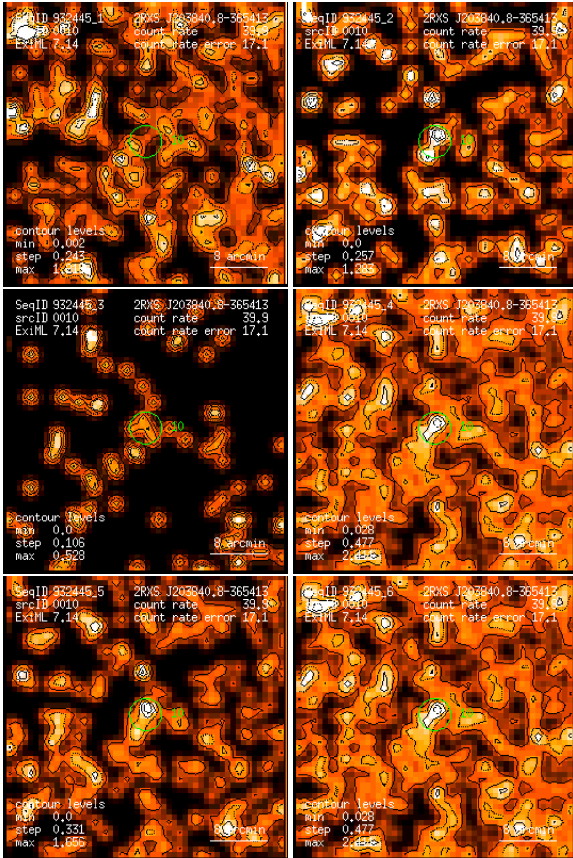
Figure 10: RASS 932445: detection 0010: band rate images, Gaussian filter: (1) PSPC channels 11 – 41, (2) 52 – 90, (3) 91 – 201, (4) 11 – 235, (5) 52 – 201, (6) 11 – 201. Broad band rates in counts/ks. Band rate contour levels in counts/ks/arcmin 2 .
