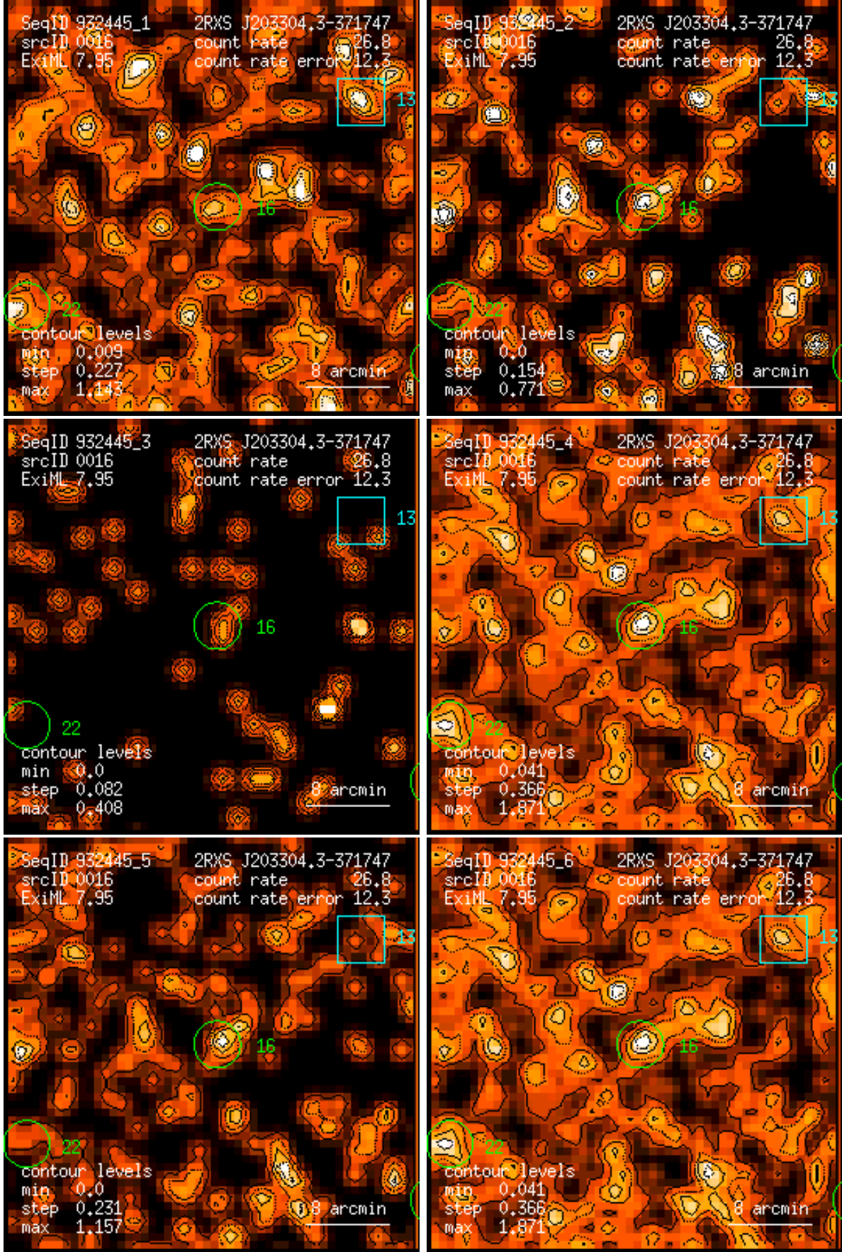
Figure 16: RASS 932445: detection 0016: band rate images, Gaussian filter: (1) PSPC channels 11 – 41, (2) 52 – 90, (3) 91 – 201, (4) 11 – 235, (5) 52 – 201, (6) 11 – 201. Broad band rates in counts/ks. Band rate contour levels in counts/ks/arcmin 2 .
