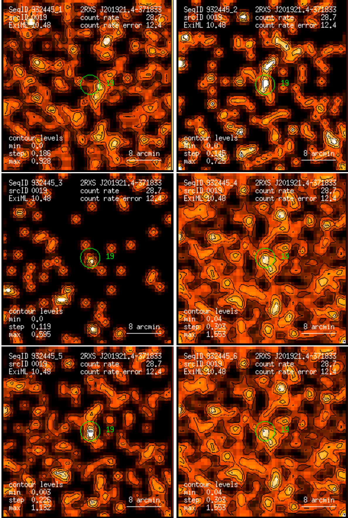
Figure 19: RASS 932445: detection 0019: band rate images, Gaussian filter: (1) PSPC channels 11 – 41, (2) 52 – 90, (3) 91 – 201, (4) 11 – 235, (5) 52 – 201, (6) 11 – 201. Broad band rates in counts/ks. Band rate contour levels in counts/ks/arcmin 2 .
