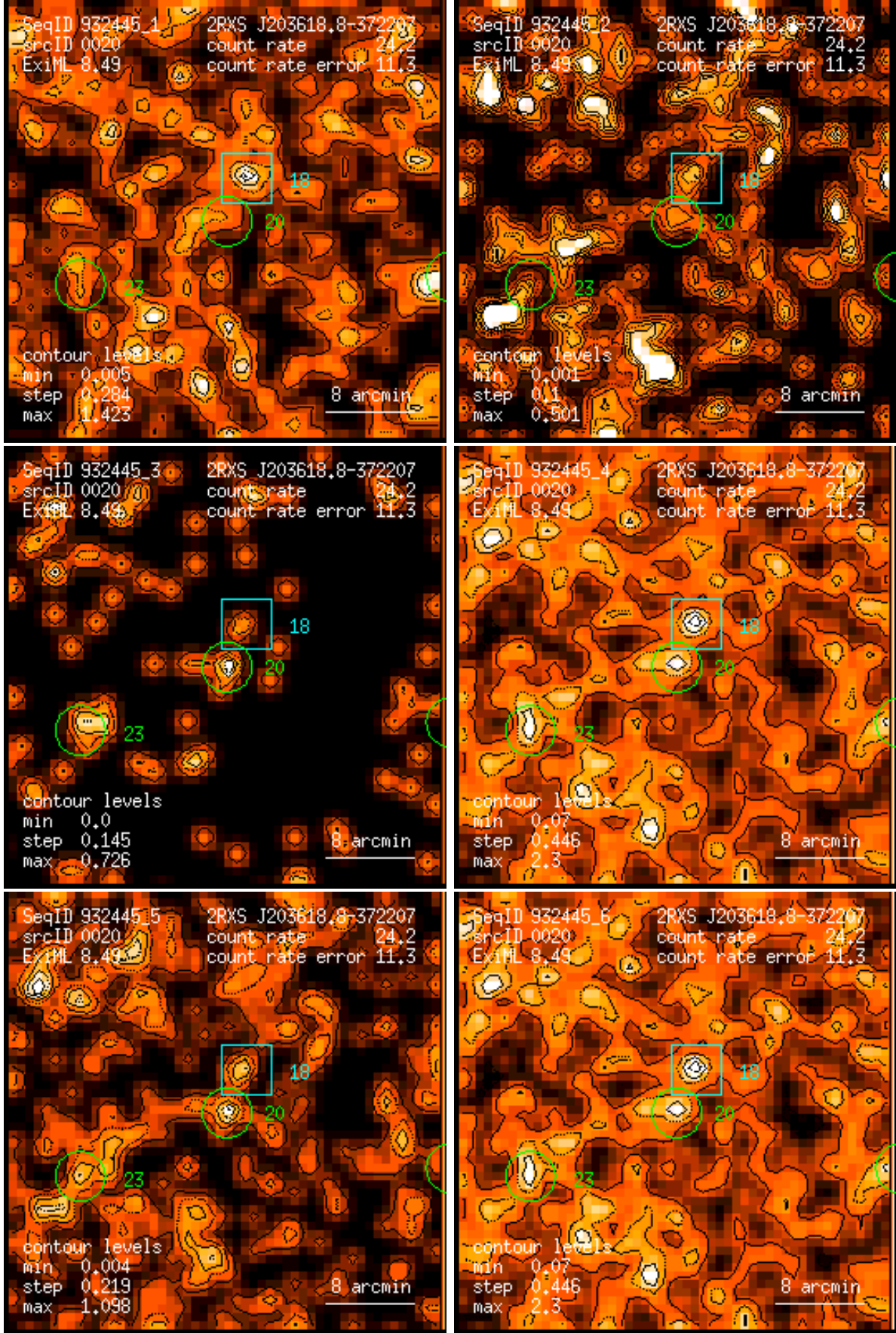
Figure 20: RASS 932445: detection 0020: band rate images, Gaussian filter: (1) PSPC channels 11 – 41, (2) 52 – 90, (3) 91 – 201, (4) 11 – 235, (5) 52 – 201, (6) 11 – 201. Broad band rates in counts/ks. Band rate contour levels in counts/ks/arcmin 2 .
