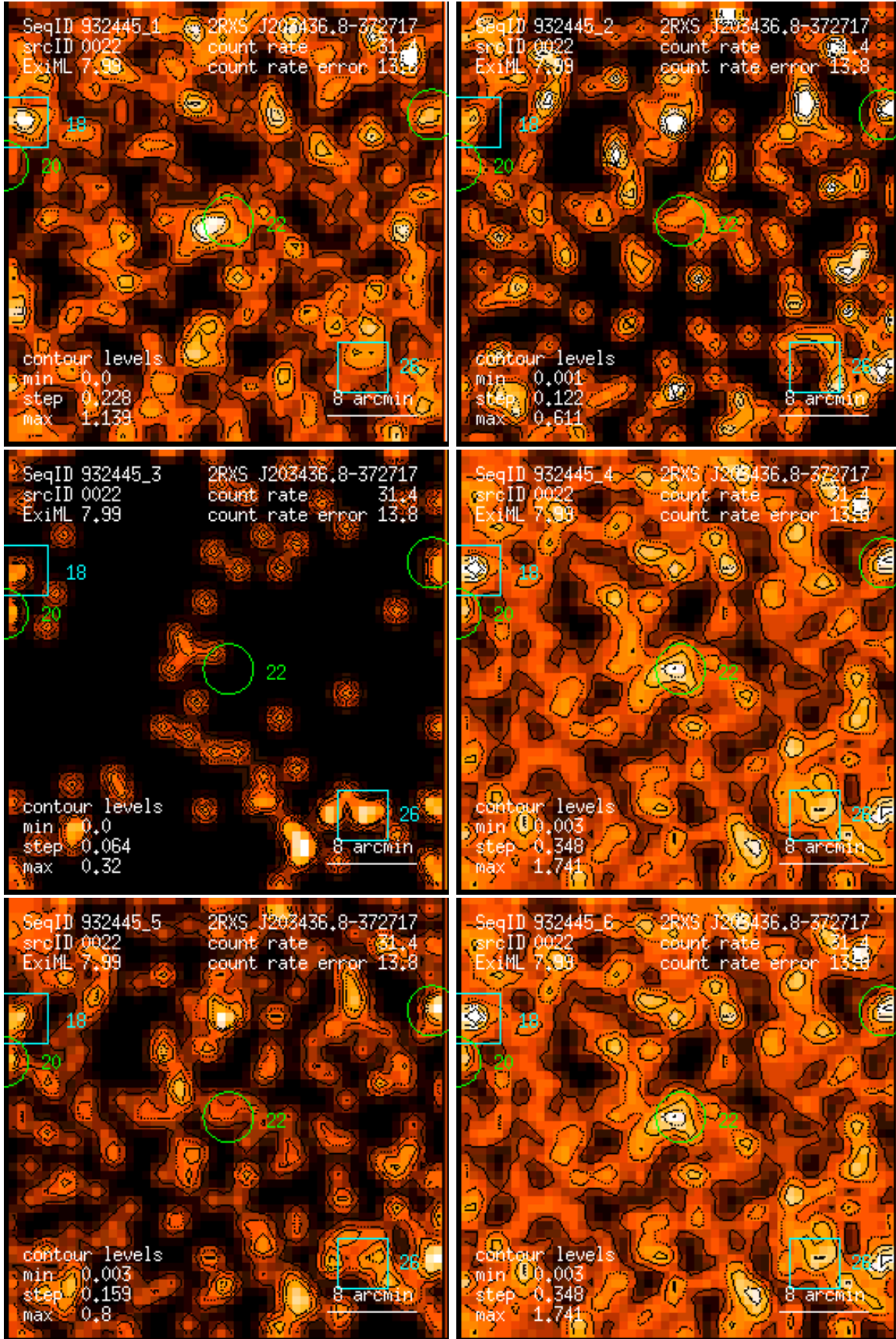
Figure 22: RASS 932445: detection 0022: band rate images, Gaussian filter: (1) PSPC channels 11 – 41, (2) 52 – 90, (3) 91 – 201, (4) 11 – 235, (5) 52 – 201, (6) 11 – 201. Broad band rates in counts/ks. Band rate contour levels in counts/ks/arcmin 2 .
