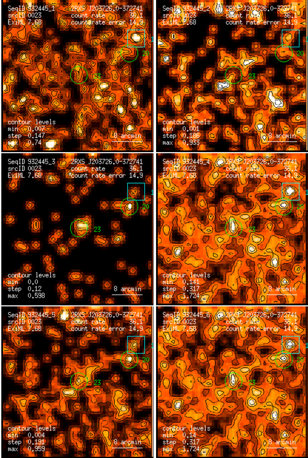
Figure 23: RASS 932445: detection 0023: band rate images, Gaussian filter: (1) PSPC channels 11 – 41, (2) 52 – 90, (3) 91 – 201, (4) 11 – 235, (5) 52 – 201, (6) 11 – 201. Broad band rates in counts/ks. Band rate contour levels in counts/ks/arcmin 2 .
