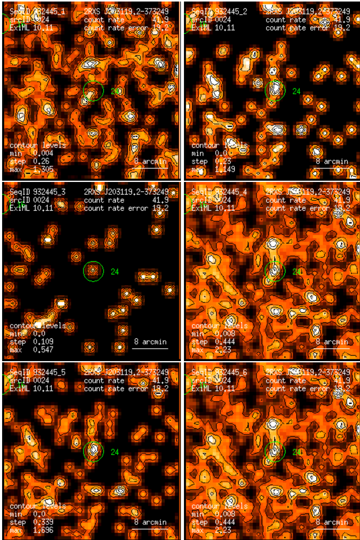
Figure 24: RASS 932445: detection 0024: band rate images, Gaussian filter: (1) PSPC channels 11 – 41, (2) 52 – 90, (3) 91 – 201, (4) 11 – 235, (5) 52 – 201, (6) 11 – 201. Broad band rates in counts/ks. Band rate contour levels in counts/ks/arcmin 2 .
