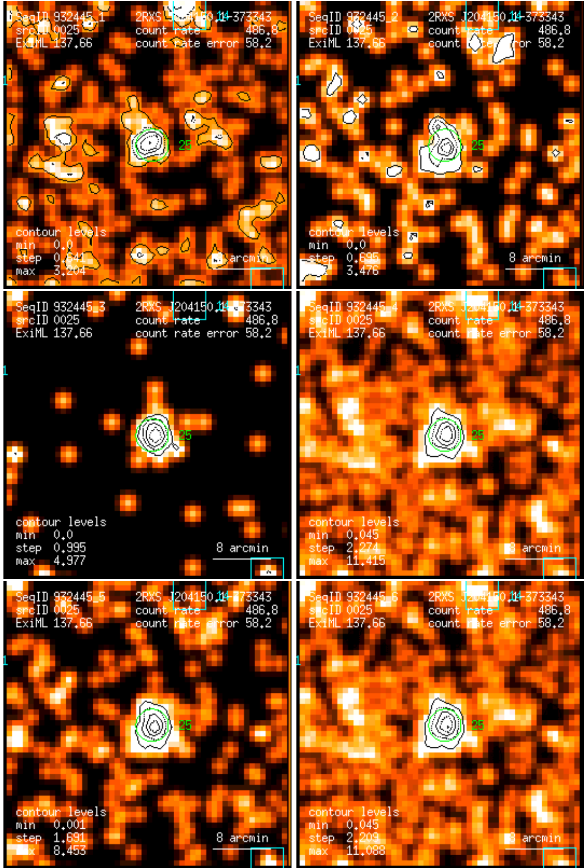
Figure 25: RASS 932445: detection 0025: band rate images, Gaussian filter: (1) PSPC channels 11 – 41, (2) 52 – 90, (3) 91 – 201, (4) 11 – 235, (5) 52 – 201, (6) 11 – 201. Broad band rates in counts/ks. Band rate contour levels in counts/ks/arcmin 2 .
