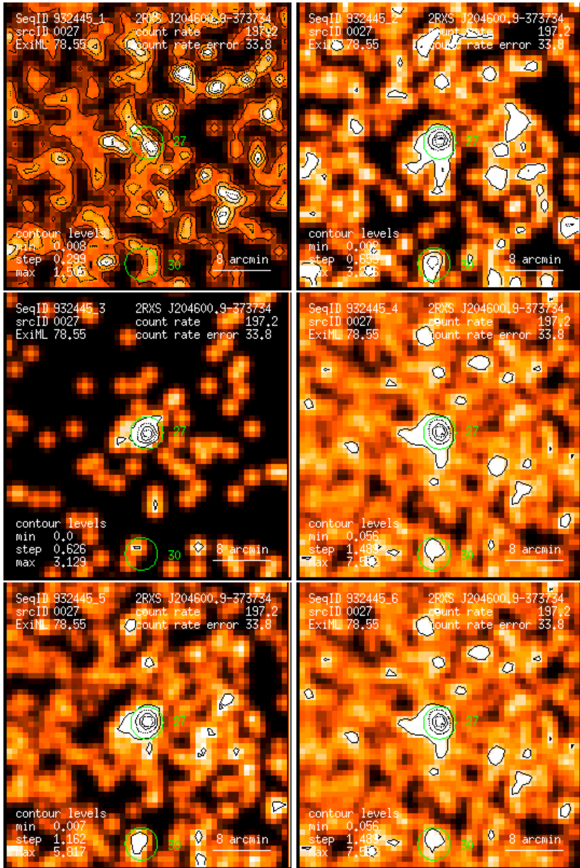
Figure 27: RASS 932445: detection 0027: band rate images, Gaussian filter: (1) PSPC channels 11 – 41, (2) 52 – 90, (3) 91 – 201, (4) 11 – 235, (5) 52 – 201, (6) 11 – 201. Broad band rates in counts/ks. Band rate contour levels in counts/ks/arcmin 2 .
