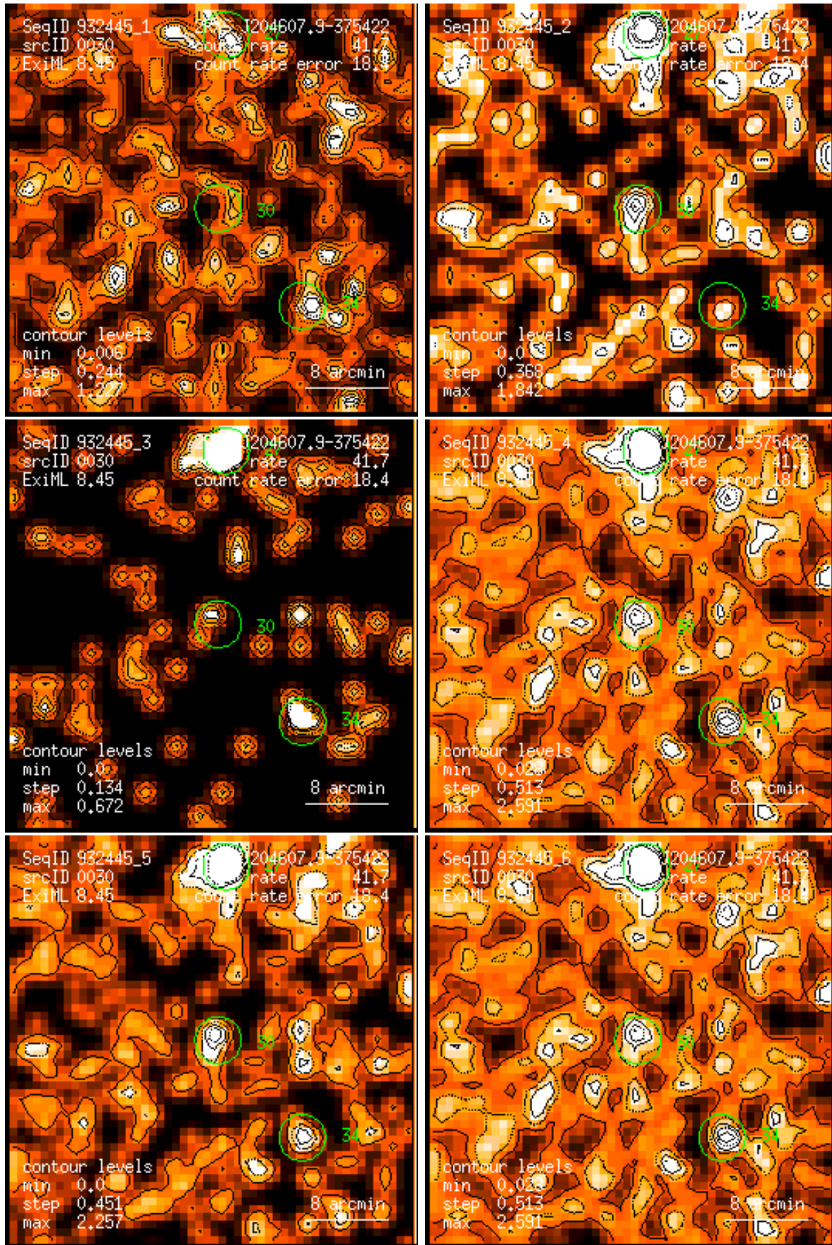
Figure 30: RASS 932445: detection 0030: band rate images, Gaussian filter: (1) PSPC channels 11 – 41, (2) 52 – 90, (3) 91 – 201, (4) 11 – 235, (5) 52 – 201, (6) 11 – 201. Broad band rates in counts/ks. Band rate contour levels in counts/ks/arcmin 2 .
