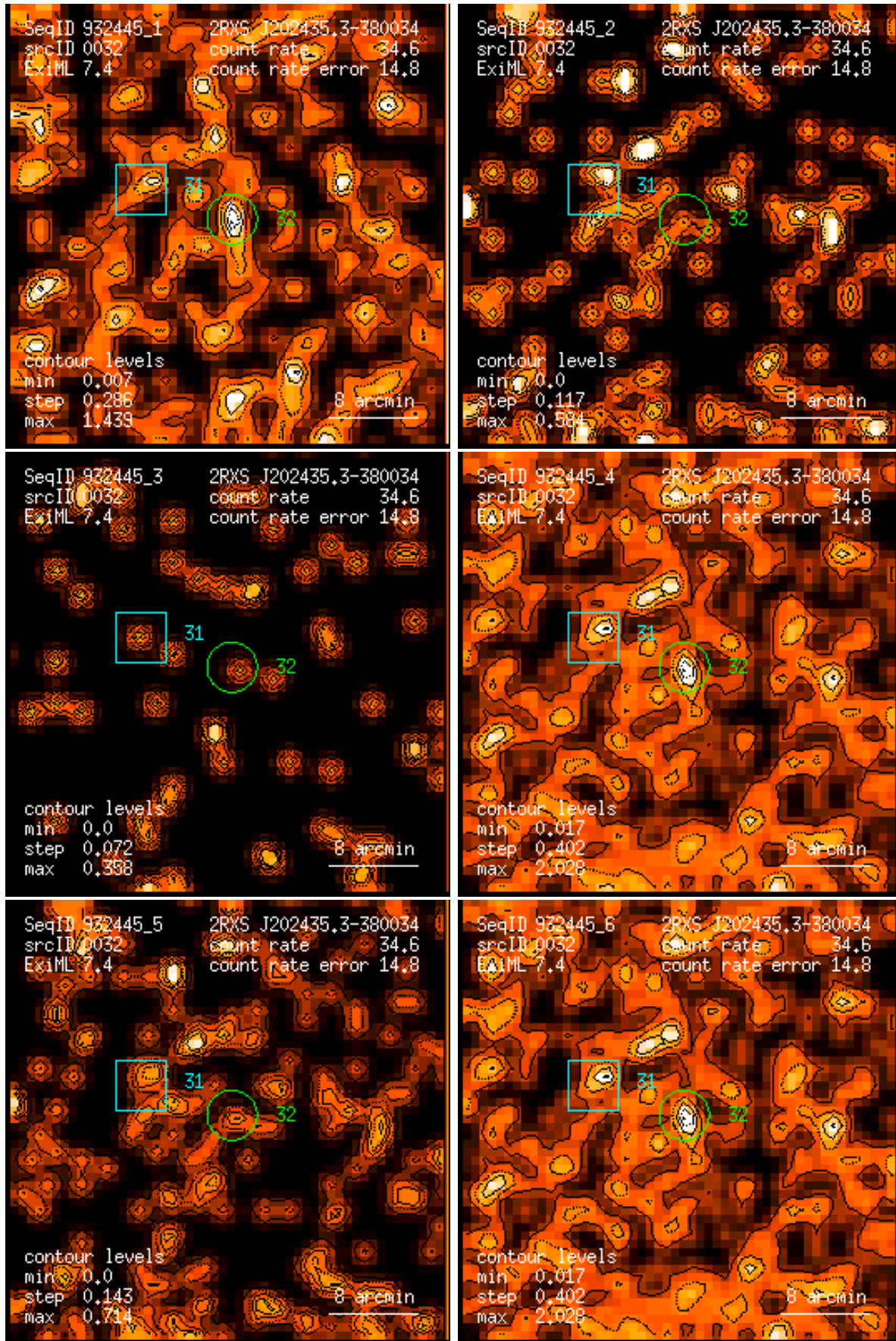
Figure 32: RASS 932445: detection 0032: band rate images, Gaussian filter: (1) PSPC channels 11 – 41, (2) 52 – 90, (3) 91 – 201, (4) 11 – 235, (5) 52 – 201, (6) 11 – 201. Broad band rates in counts/ks. Band rate contour levels in counts/ks/arcmin 2 .
