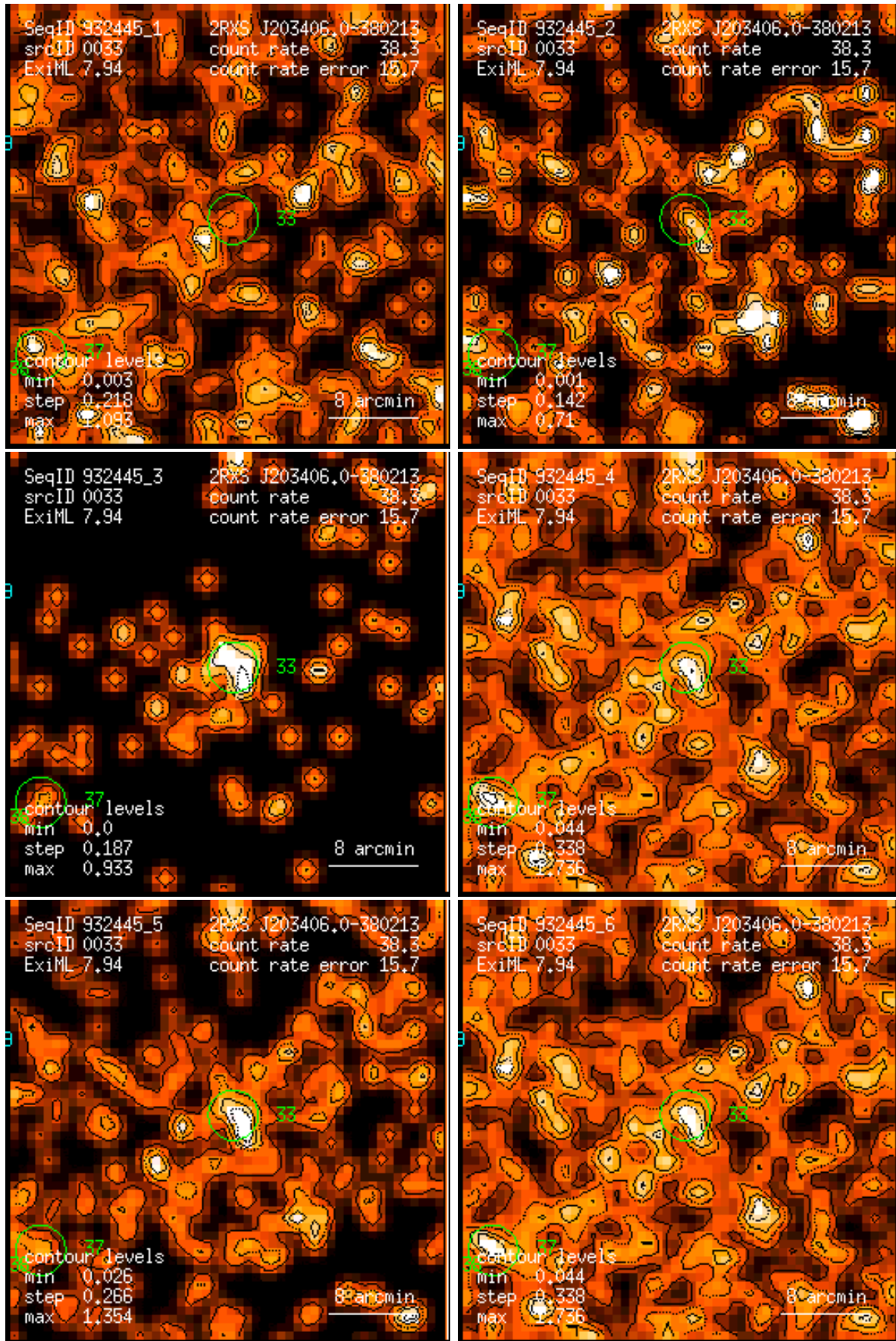
Figure 33: RASS 932445: detection 0033: band rate images, Gaussian filter: (1) PSPC channels 11 – 41, (2) 52 – 90, (3) 91 – 201, (4) 11 – 235, (5) 52 – 201, (6) 11 – 201. Broad band rates in counts/ks. Band rate contour levels in counts/ks/arcmin 2 .
