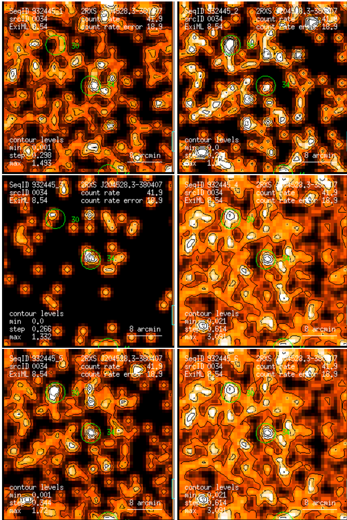
Figure 34: RASS 932445: detection 0034: band rate images, Gaussian filter: (1) PSPC channels 11 – 41, (2) 52 – 90, (3) 91 – 201, (4) 11 – 235, (5) 52 – 201, (6) 11 – 201. Broad band rates in counts/ks. Band rate contour levels in counts/ks/arcmin 2 .
