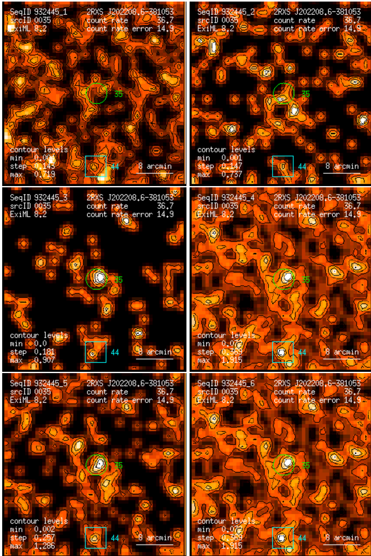
Figure 35: RASS 932445: detection 0035: band rate images, Gaussian filter: (1) PSPC channels 11 – 41, (2) 52 – 90, (3) 91 – 201, (4) 11 – 235, (5) 52 – 201, (6) 11 – 201. Broad band rates in counts/ks. Band rate contour levels in counts/ks/arcmin 2 .
