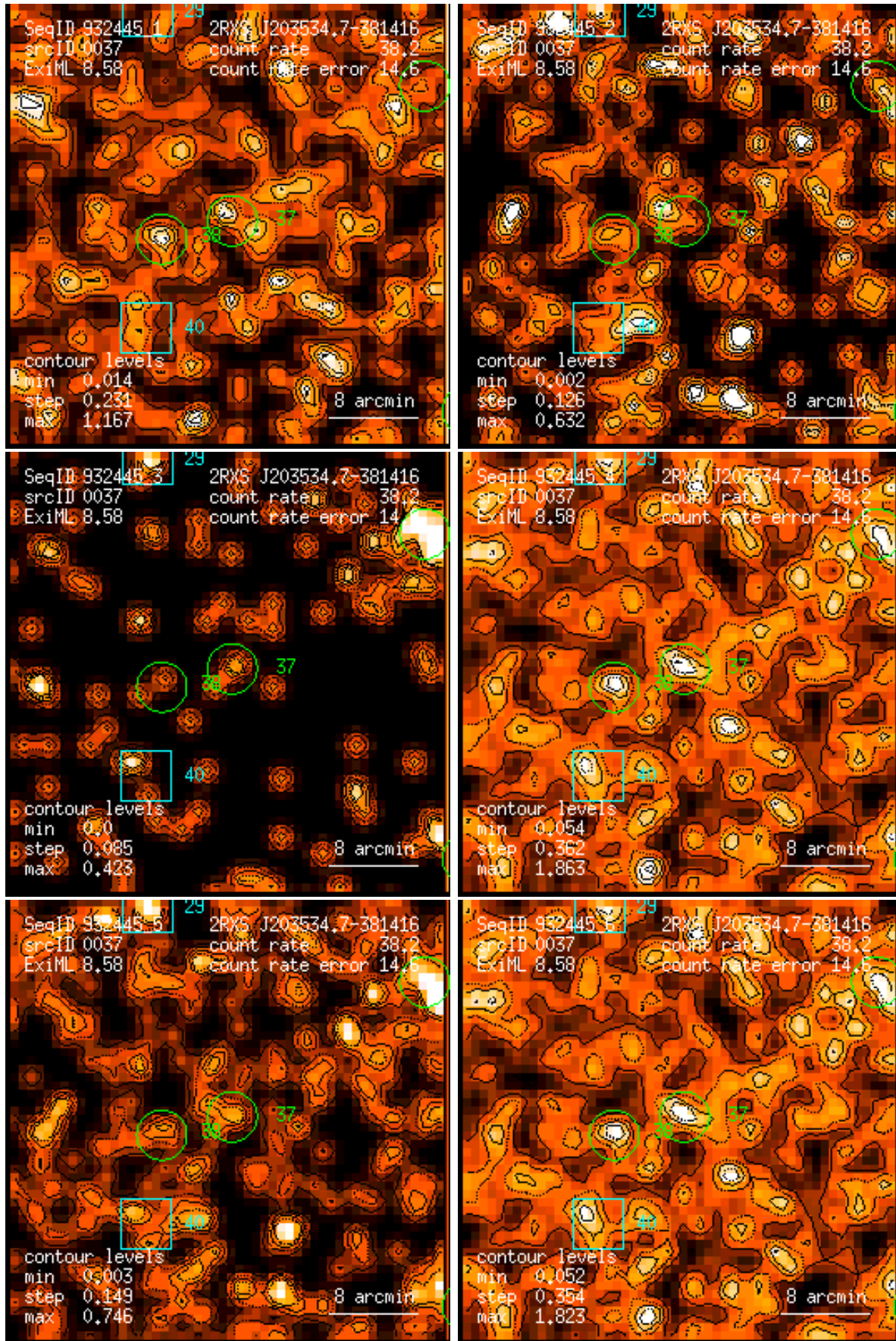
Figure 37: RASS 932445: detection 0037: band rate images, Gaussian filter: (1) PSPC channels 11 – 41, (2) 52 – 90, (3) 91 – 201, (4) 11 – 235, (5) 52 – 201, (6) 11 – 201. Broad band rates in counts/ks. Band rate contour levels in counts/ks/arcmin 2 .
