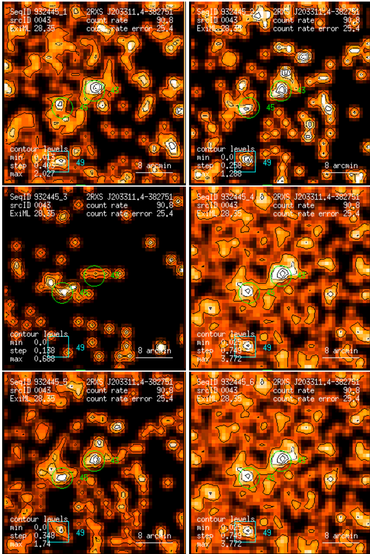
Figure 43: RASS 932445: detection 0043: band rate images, Gaussian filter: (1) PSPC channels 11 – 41, (2) 52 – 90, (3) 91 – 201, (4) 11 – 235, (5) 52 – 201, (6) 11 – 201. Broad band rates in counts/ks. Band rate contour levels in counts/ks/arcmin 2 .
