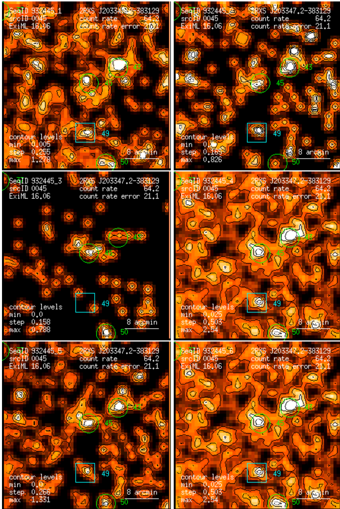
Figure 45: RASS 932445: detection 0045: band rate images, Gaussian filter: (1) PSPC channels 11 – 41, (2) 52 – 90, (3) 91 – 201, (4) 11 – 235, (5) 52 – 201, (6) 11 – 201. Broad band rates in counts/ks. Band rate contour levels in counts/ks/arcmin 2 .
