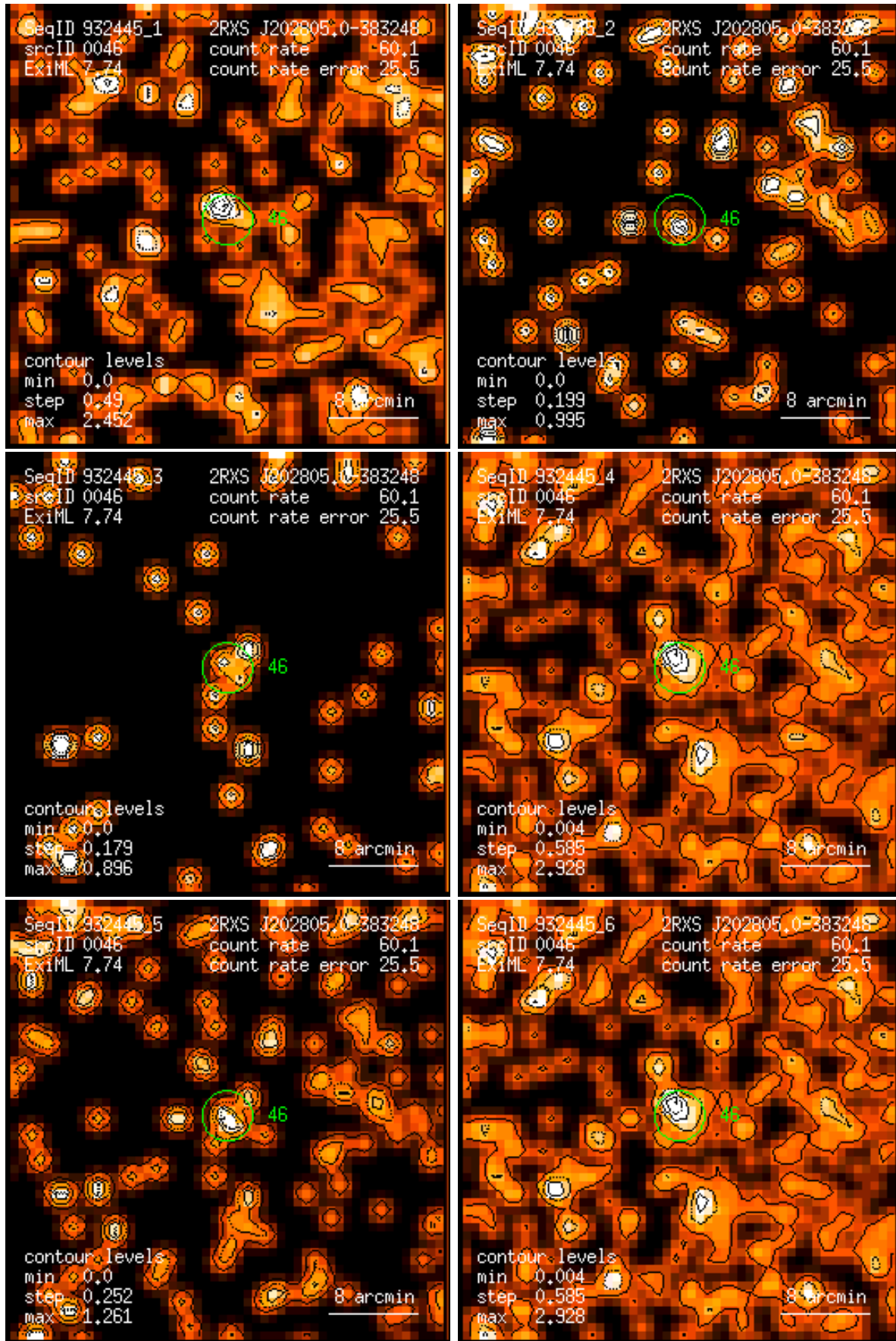
Figure 46: RASS 932445: detection 0046: band rate images, Gaussian filter: (1) PSPC channels 11 – 41, (2) 52 – 90, (3) 91 – 201, (4) 11 – 235, (5) 52 – 201, (6) 11 – 201. Broad band rates in counts/ks. Band rate contour levels in counts/ks/arcmin 2 .
